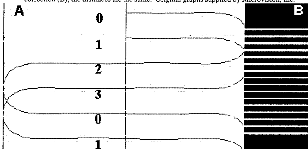
Figure 3. Line numbering and pattern for evaluating line pairs. (A) Graph of dual scanning with pinch correction. The lines are numbered 0, 1, 2, 3, depicting the four line conditions. (B) Horizontal grill pattern comprised of 2 lines followed by five lines off and the pattern repeated. Original graph (A) supplied by Microvision, Inc.
