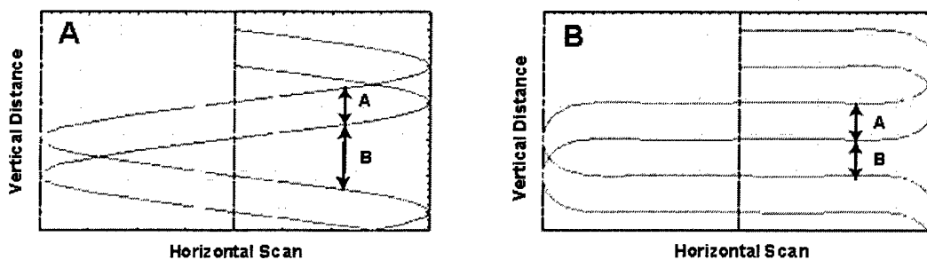
Figure 2. Graphs of scanned lines representing dual scans with no pinch correction (A) and dual scans with pinch correction (B). Note the difference between distance A and B in (A), whereas with pinch correction (B), the distances are the same. Original graphs supplied by Microvision, Inc.
