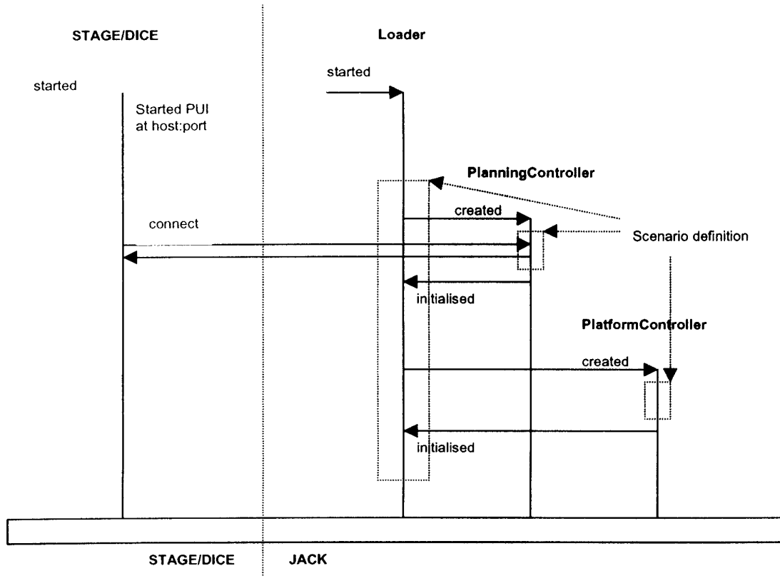
Figure A-2: Startup Event Flow.
