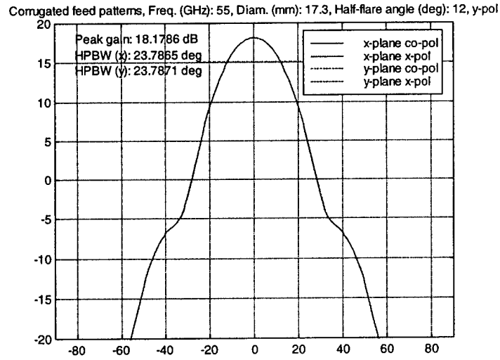
Figure 4(b). 55 GHz Feed pattern
