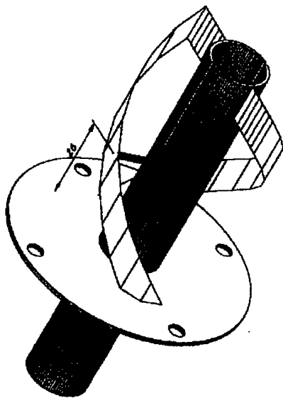
Figure 2, Model 4 “S” Band Modified Kilgus Antenna Prototype
