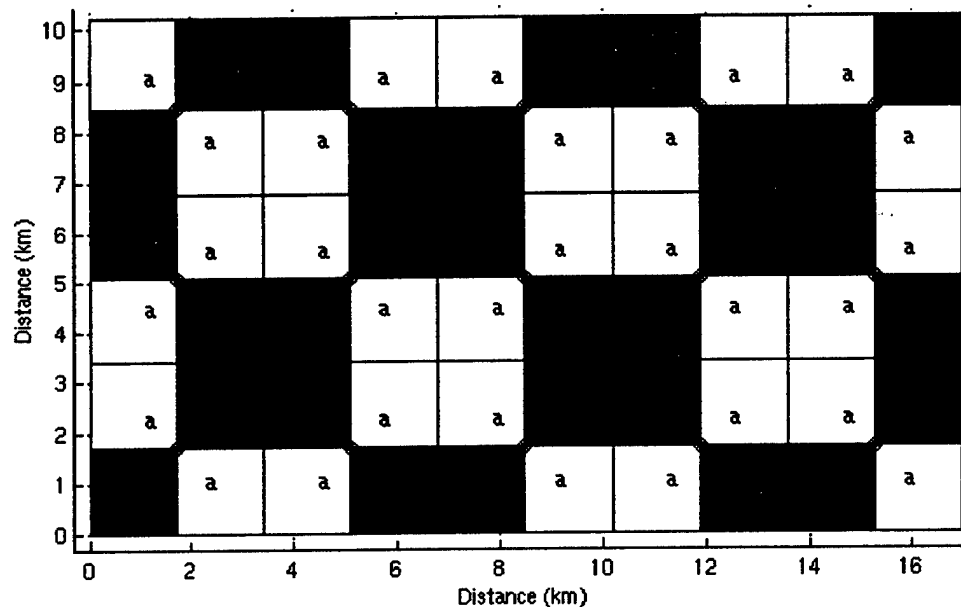
Fig. 9 A square cell plan with 3 by 5 radio hubs indicated with ⊗. Upper (dark) and lower (light) cases represent orthogonal polarization directions that use the same frequency.
