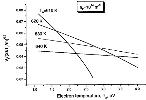
Figure 2. The velocity V_1 as a function of plasma temperature with Teflon surface temperature as a parameter.
