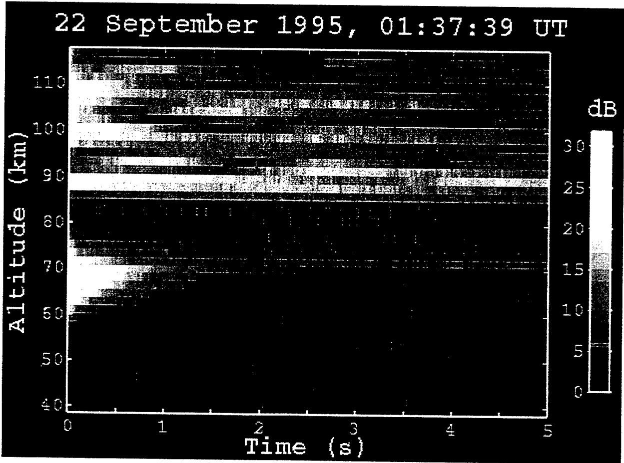
Figure 6. API measured at the beginning of a power stepping sequence with 40 MW ERP.
