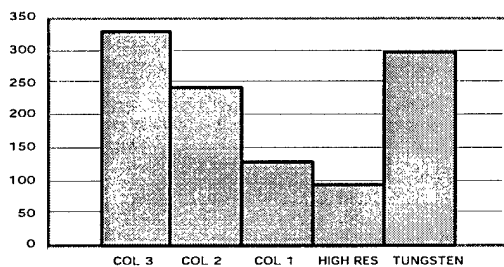
Figure 5: Comparative sensitivity measured for five selected collimators for \pm 10\% energy window.
