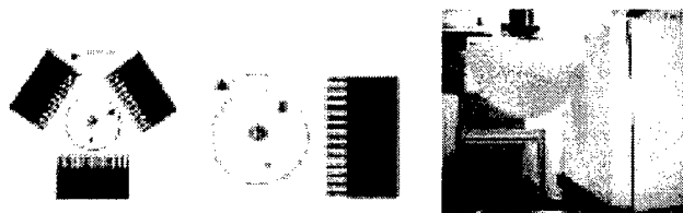
Figure 14: SPECT geometry. The left schematic shows the concept of an optimized 3-head system. In the tests the breast phantom was rotated in front of a single detector (a 4"x4" camera is shown in this example).
