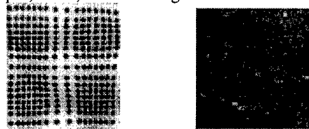
Figure 4: Left: A four PSPMT region of the raw image obtained with a \text{Na}^{22} source. Each scintillator pixel is well separated. Note the spatial distortion due to the combined effects of the dead regions between the PSPMTs and the non uniformity of gain characteristics of the individual photomultipliers. Right: A Corrected image of the same region.
