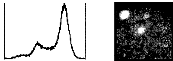
Figure 9: Left: An example of the energy spectrum measured for \text{Tc}^{99\text{m}} with a compressed breast phantom from figure 8. Right: Uniformity and flood corrected non-filtered image of the same phantom using a -2.5%-to-+30% energy window around the center of photopeak.
