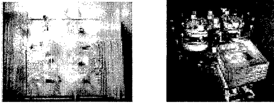
Figure 7a: Left: Top view of the multi-lesion breast box phantom. Right: View of the phantom attached to the torso during imaging session. Small gamma camera is placed below the phantom.
