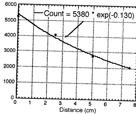
Figure 12: Dependence of detection sensitivity, expressed in counts per 10 minutes within lesion ROI as a function of lesion distance from detector (in cm). Hot 9mm diameter lesion in a cold breast phantom filled with water was used.
