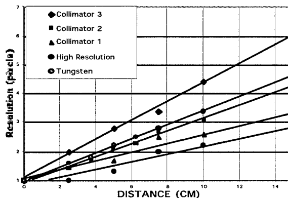
Figure 6: System resolution with various collimators. Each of lines represents a linear fit through the data points. Vertical scale is in scintillation pixels (1 pixel = 3.3 mm).
