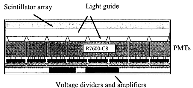
Figure 1: Schematic of the detector head of an array of 8x6 R7600-00-C8 PSPMTs. (Collimator and tungsten shield are not shown.)
