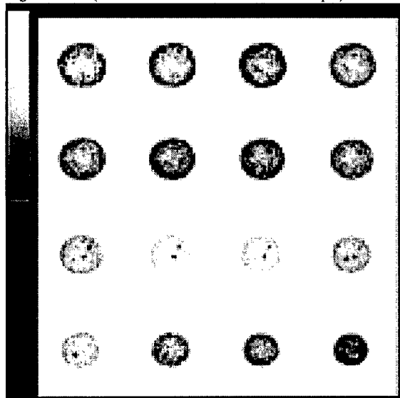
Figure 15: Example of the SPECT reconstruction results obtained with a 8"x6" imager prototype. Sixteen 3.3mm slices are shown. Left top slice #1 is the closest to the base of the breast phantom, the bottom right slice #16 is the closest to the "nipple" region. Slice #12 shows all three lesions.
