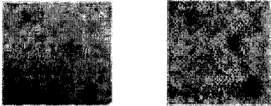
Figure 7b: Left: 5 minute CsI(Tl) detector unfiltered image of the multi-lesion breast box phantom with the high intensity flood phantom ("hot torso") against bottom edge. Right: NaI(Tl) detector image under identical conditions.
