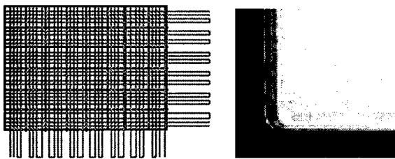
Figure 3: Left: an 8 \times 6 PSPMT diagram demonstrating combined wire readout approach with decoupled edge wires resulting in the 18 \times 14 channel readout. Right: A photographic zoom of the corner region of the 8'' \times 6'' NaI(Tl) crystal array. Note the minimized dead space at the bottom edges (chest wall side).
