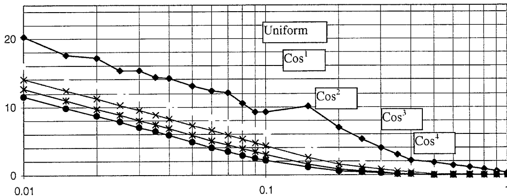
Figure 3: Near-Field Correction Factors for Rectangular Aperture
