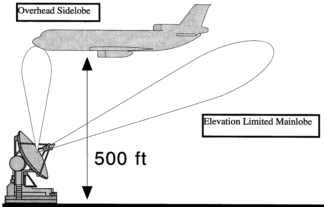
Figure 6: Illustration of Overhead Illumination
