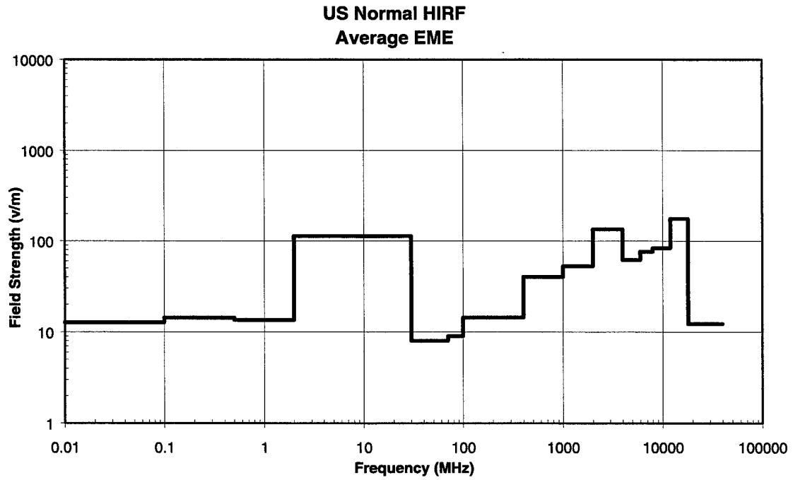
Figure 16: Average U.S. Normal Environment
