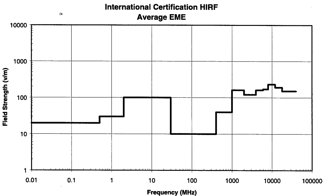
Figure 30: Average International Certification Environment
