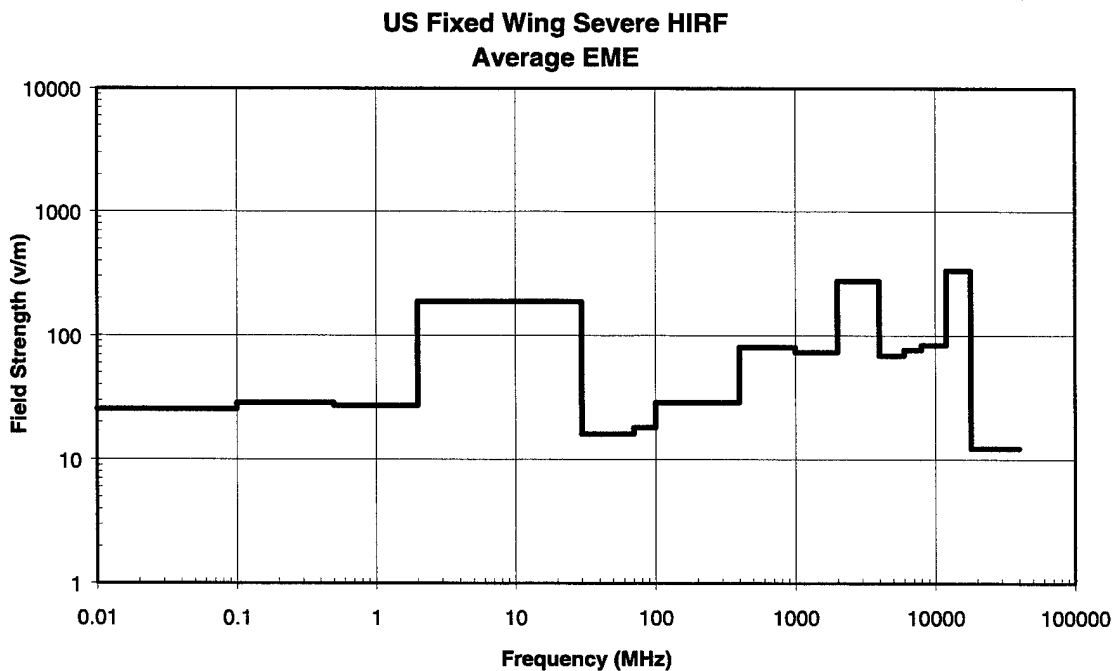
Figure 12: Average U.S. Fixed Wing Severe Environment
