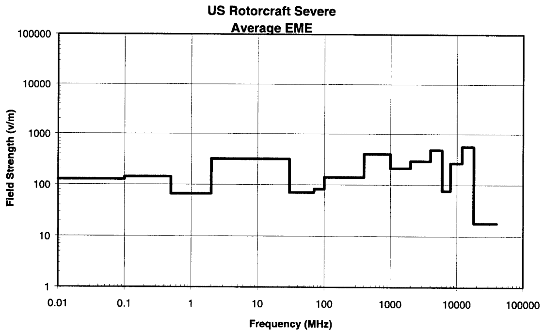
Figure 10: Average U.S. Rotorcraft Severe Environment
