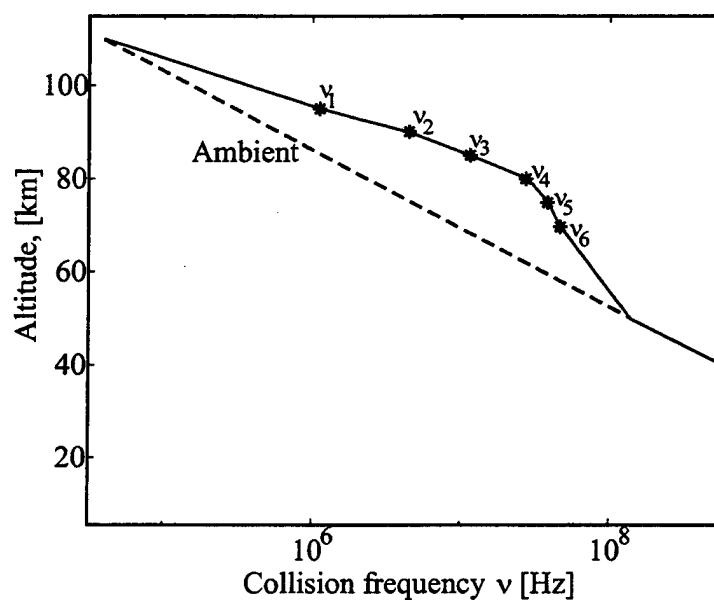
Figure 4.2: Collision frequency profile is modeled with six different values of collision frequency at six different altitudes in the D -region. The altitude range sampled is chosen on the basis of the sensitivity of the subionospheric VLF signal to changes at different altitudes.
