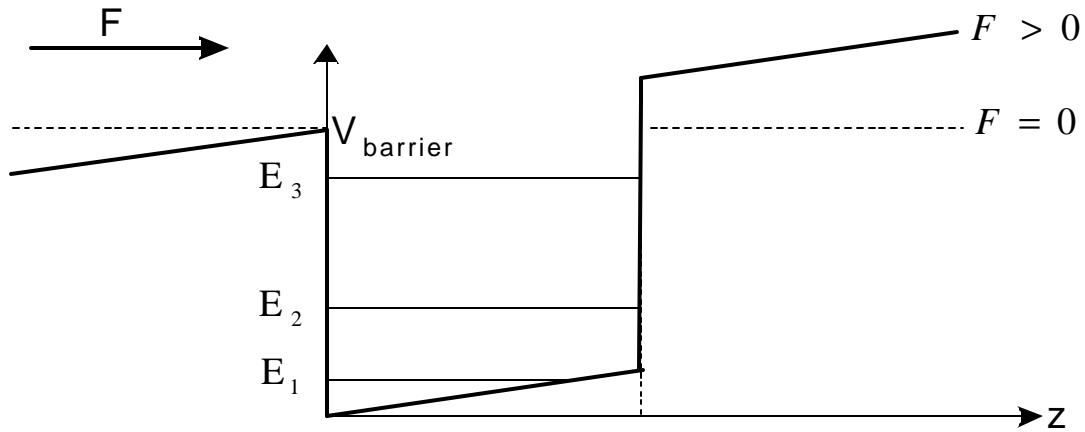
Figure 2.11 Schematic representation of a square quantum well under an applied bias.
