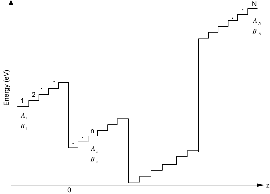
Figure 2.13 The stair case approximation of the potential shown in Figure 2.12.
