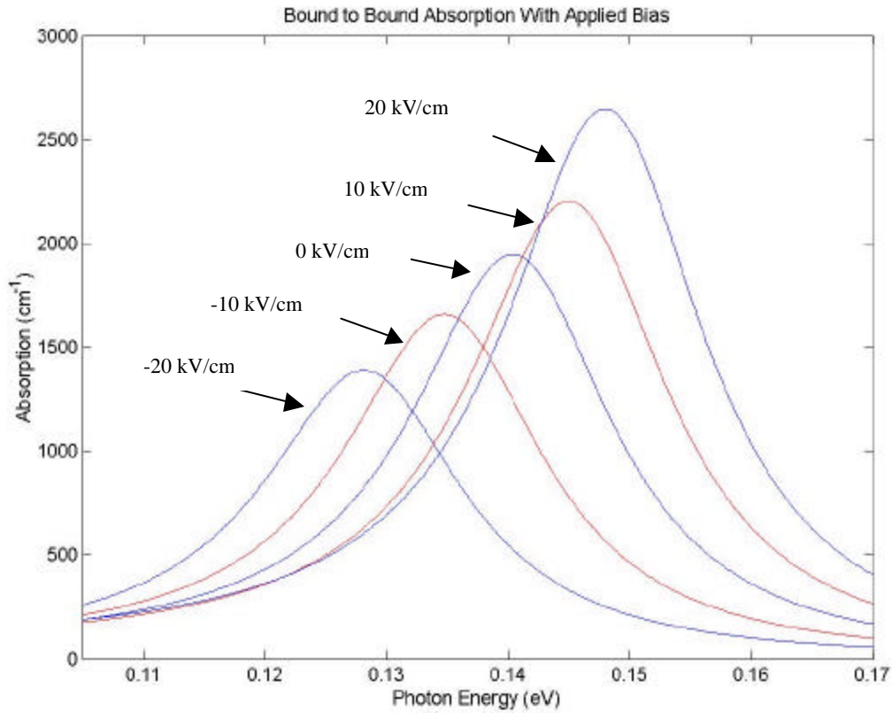
Figure 4.2 Absorption coefficient for bound-to-bound intersubband transition for the step well shown in Figure 4.1 for a set of bias voltages.
