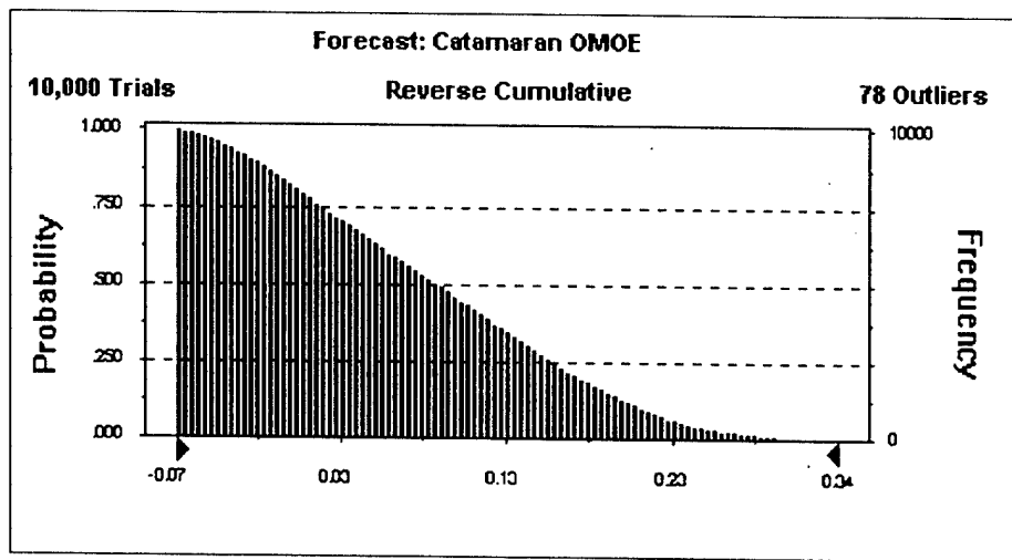
Figure 19: Catamaran OMOE Reverse Cumulative Chart (Payload = 100 Iton, Speed = 35 kts, Range = 1000 nm)
