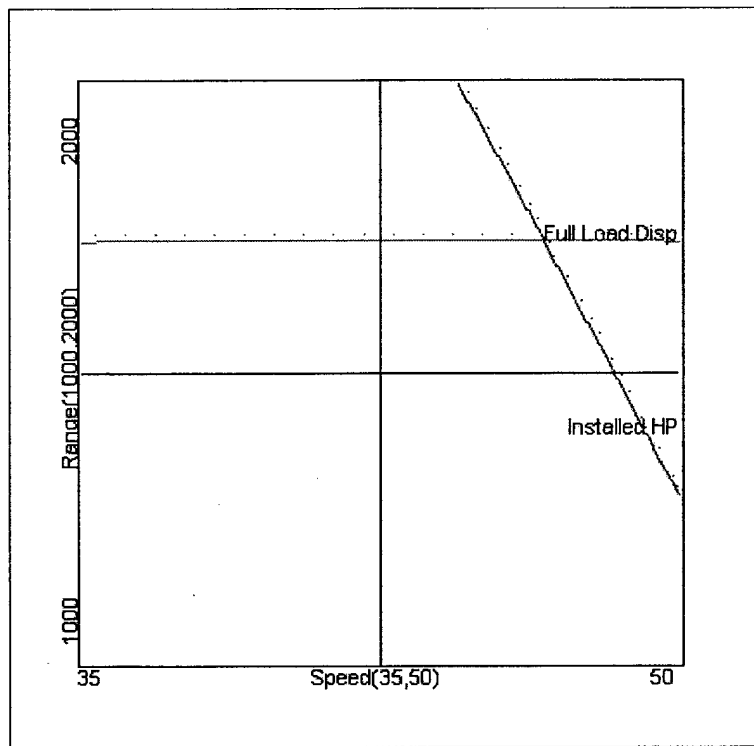
Figure 14: Catamaran Contour Plot (Payload = 150 tton, Full Load Displacement = 750 tton, Installed Power = 28,000 hp)
