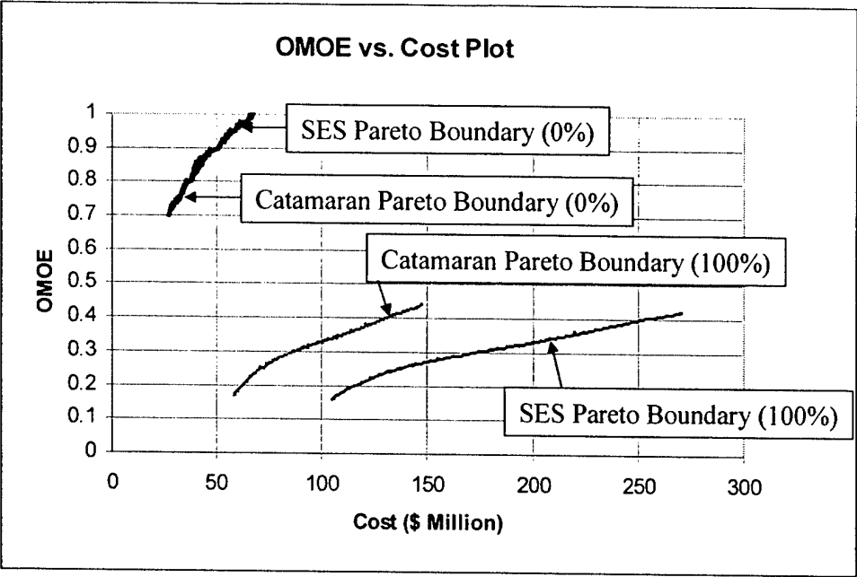
Figure 23: OMOEO vs. Cost Plot showing Pareto Boundaries
