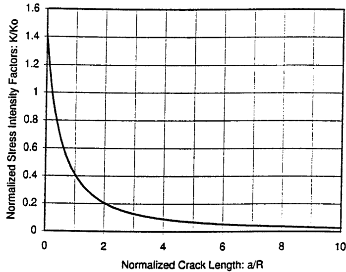
Figure 7. A Crack Emanating from a Hole under a Pair of Point Loads: K_o = \frac{F}{2Rt} \sqrt{\pi a}
