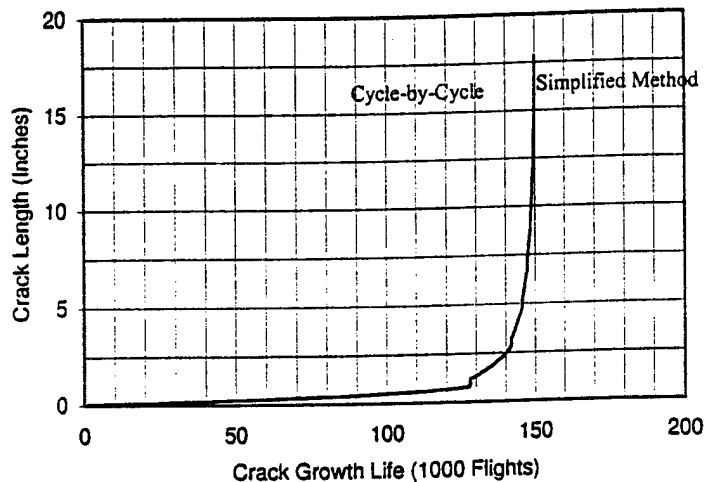
Figure 6. Crack Growth Life of the Example Repair
