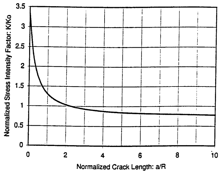
Figure 6. A Crack Emanating from a Hole under Uniform Far Field Stress: K_0 = \sigma_\infty \sqrt{\pi a}
