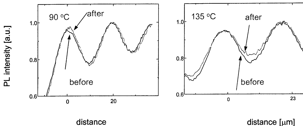
Figure 59. Spatial PL intensity profiles before and after 4 hour anneal at 90 °C or 135 °C of substrates with C6 stripes patterns diffused into PVK/PBD film.
