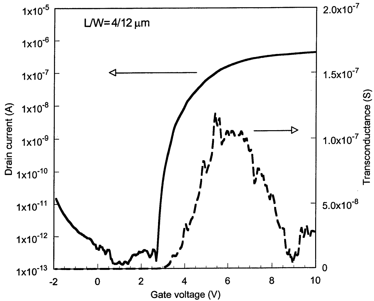
Figure 2. Transfer characteristics and transconductance of as-processed mc-Si TFTs when V_d = 1\text{V} . The substrate temperatures were maintained below 285^\circ\text{C} during the HDP depositions.
