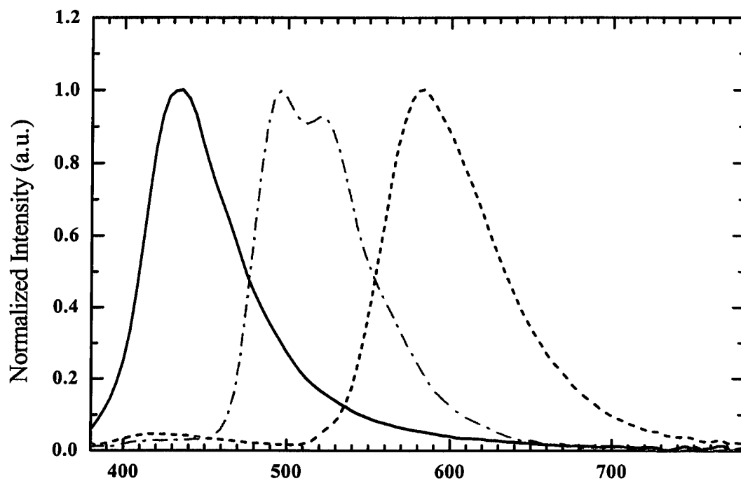
Figure 64. EL emission in RGB pixels using respectively a device polymer of PVK doped uniformly with C47 (blue), with patterned Nile Red, patterned C6, and no added patterned dopant, respectively. [26]
