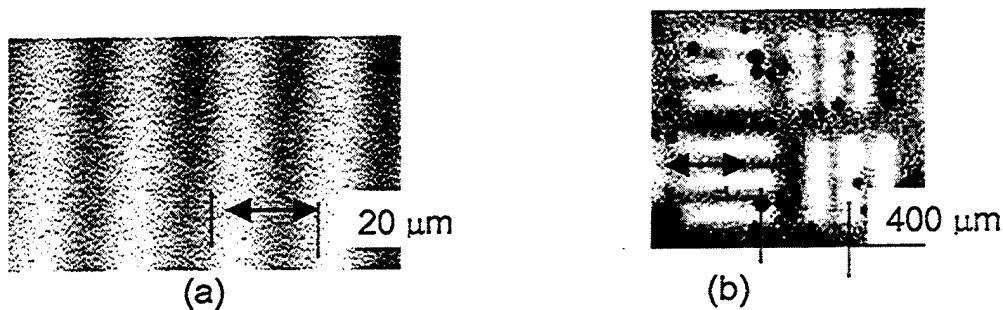
Figure 56. (a) PL micrograph and (b) EL micrograph of lines with C6 diffused into a film of PVK/PBD using a transferred photoresist mask
