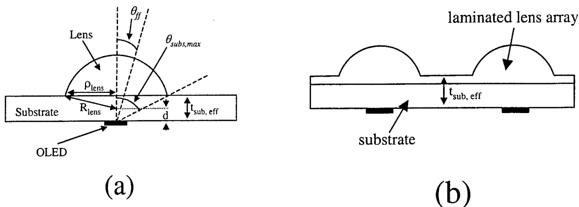
Figure 66. Use of spherical surface features to improve external efficiency. The relevant parameters shown are given for each experimental trial in Table 1. Note that the ray used to define the far-field angle, \theta_{\text{ff}} , is drawn for the d=0 case, while in the diagram d , the offset between the center of curvature of the lens and the OLED, is drawn as non-zero so that it can be clearly identified. (b) Spherical features implemented as a plastic lens array laminated to a planar substrate. [9]
