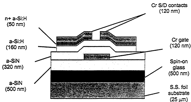
Figure 24. Cross-sectional schematic of a-Si TFT on planarized substrate of stainless steel foil.
