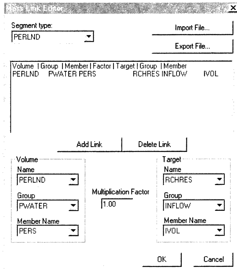
Figure 8. Mass Link Editor
