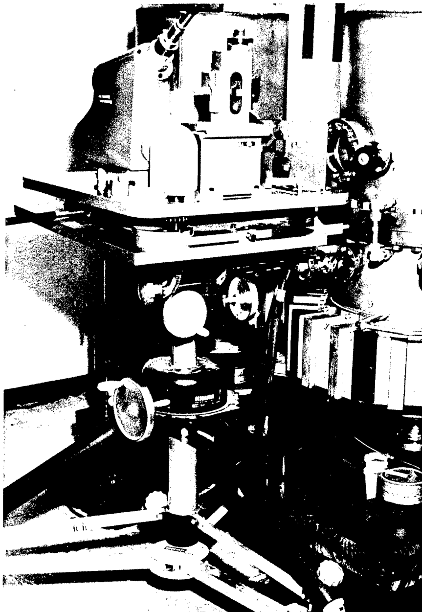
FIGURE 8 OPTICAL EXTENSOMETER
