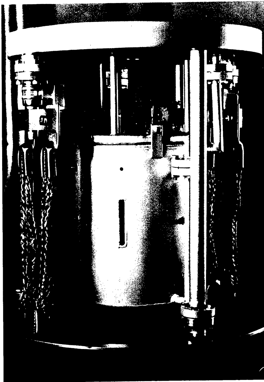
FIGURE 5 CREEP UNIT WITH BELL REMOVED SHOWING BRIDGE AND COLDWALL FURNACE
