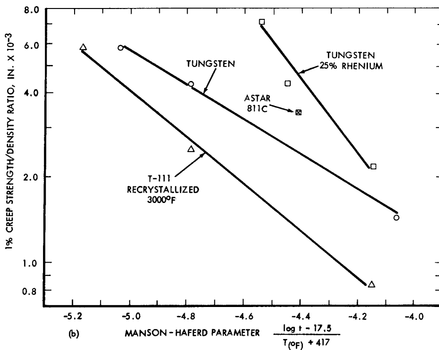
FIGURE 101 PARAMETRIC COMPARISON OF ASTAR 811C, ARC MELTED TUNGSTEN, TUNGSTEN-25% RHENIUM AND T-111 SHEET; a) 1% CREEP STRENGTH, b) 1% CREEP STRENGTH-TO-DENSITY RATIO.
