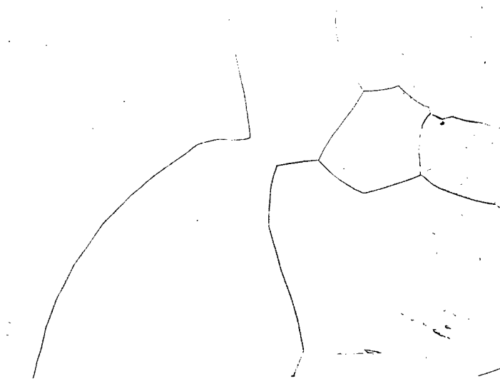
FIGURE 89 GRAIN GROWTH IN ARC MELTED TUNGSTEN CREEP SPECIMEN S-9 TESTED 3886 HOURS AT 3200°F (1670°C). ETCHANT: 15% HF, 15% H 2 SO 4 , 8% HNO 3 , 62% H 2 O. 100 X
