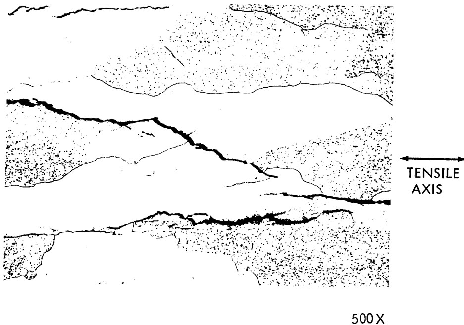
FIGURE 57 PHOTOMICROGRAPHS OF CRACK IN TZC (HEAT M-91) SPECIMEN B-22. ETCHANT: 15% HF, 15% H_2SO_4 , 8% HNO_3 , 62% H_2O .
