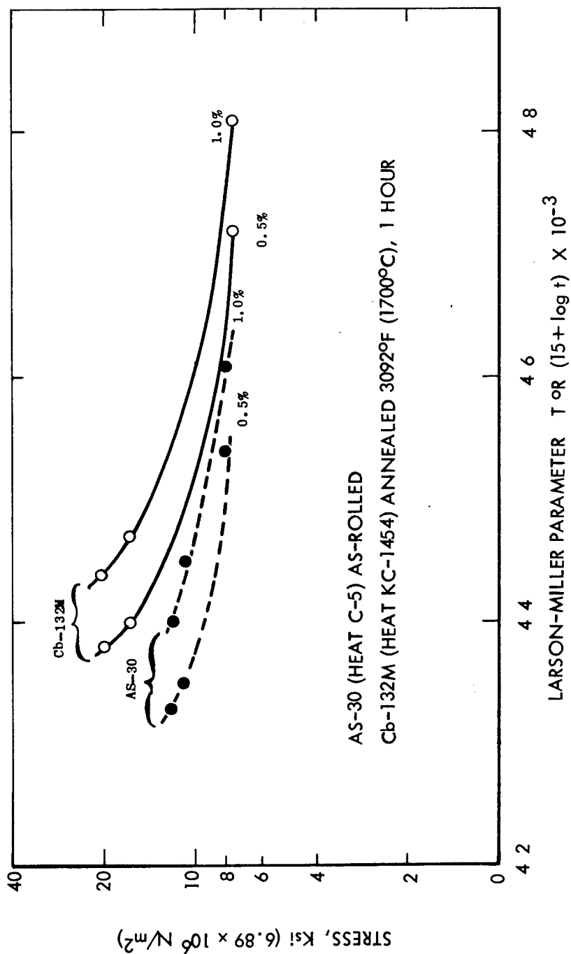
FIGURE 48 LARSON-MILLER PLOT FOR 0.5 AND 1.0% CREEP IN AS-30 AND Cb-132M PLATE. TESTED IN VACUUM ENVIRONMENT < 1 \times 10^{-8} TORR.
