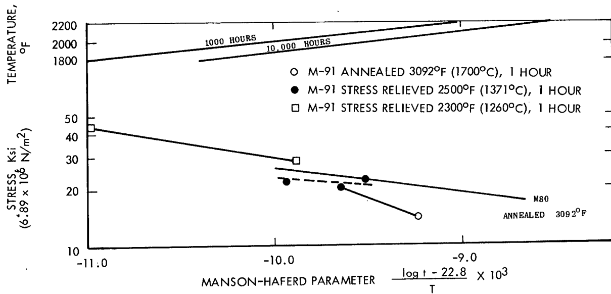
FIGURE 59 PARAMETRIC PLOTS OF 0.5% CREEP DATA FOR TZC PLATE. TESTED IN VACUUM ENVIRONMENT < 1 \times 10^{-8} TORR.
