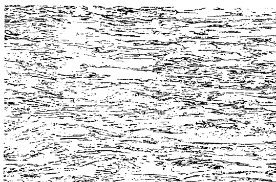
FIGURE 25 PHOTOMICROGRAPHS SHOWING ETCHED SECTIONS OF TZM PANCAKE-FORGED DISC (HEAT 7502) IN AS-RECEIVED CONDITION. ETCHANT: MURAKAMI'S. 100X
