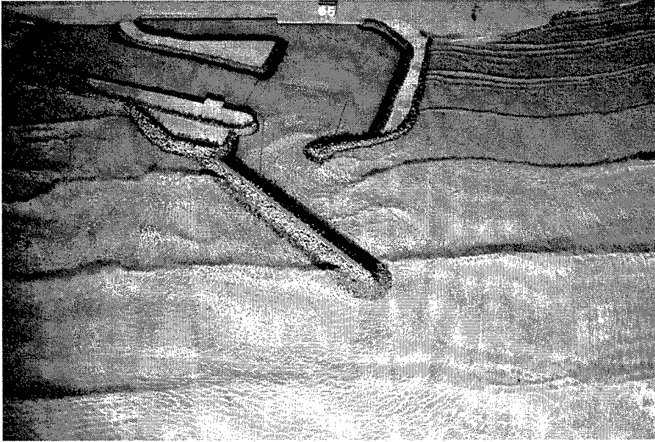
Photo 33. Typical wave patterns for Alternative 1d; 8-sec, 3-ft waves from 160 deg; swl = +1.0 ft mlw
