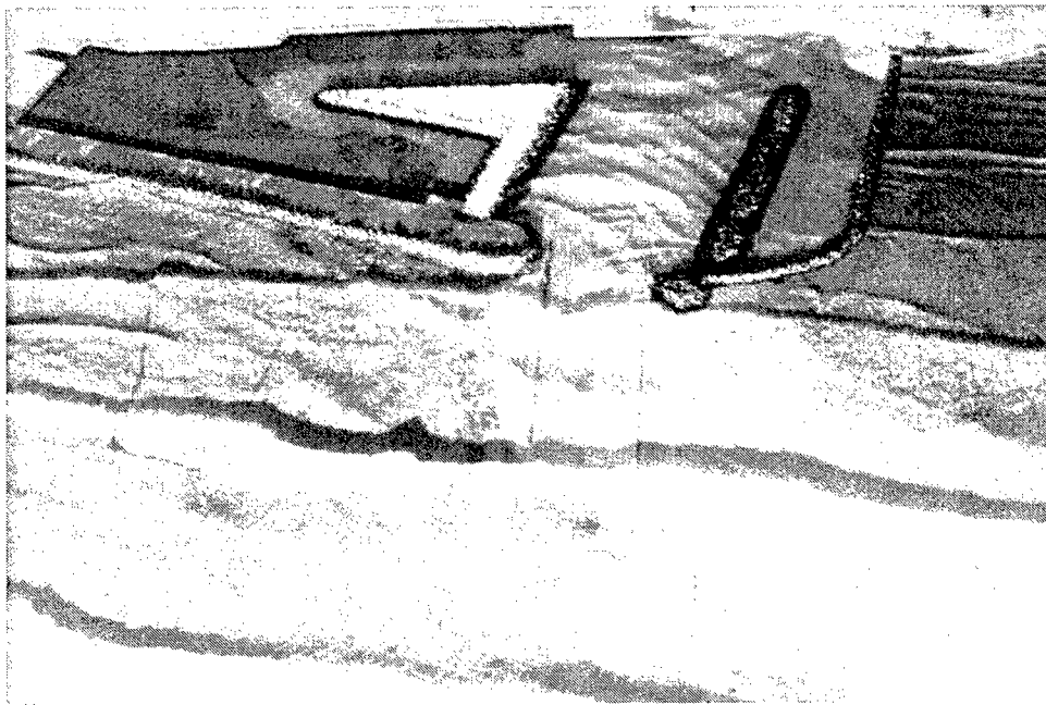
Photo 60. Typical wave patterns for Alternative 8; 14-sec, 6-ft waves from 180 deg; swl = +1.0 ft mlw
