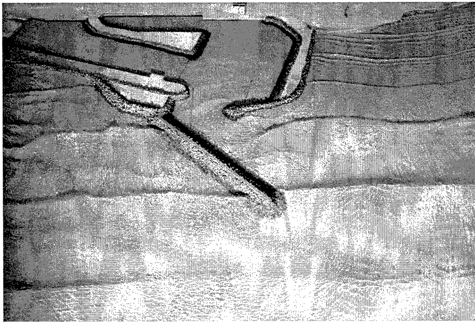
Photo 34. Typical wave patterns for Alternative 1d; 14-sec, 6-ft waves from 160 deg; swl = +1.0 ft mlw
