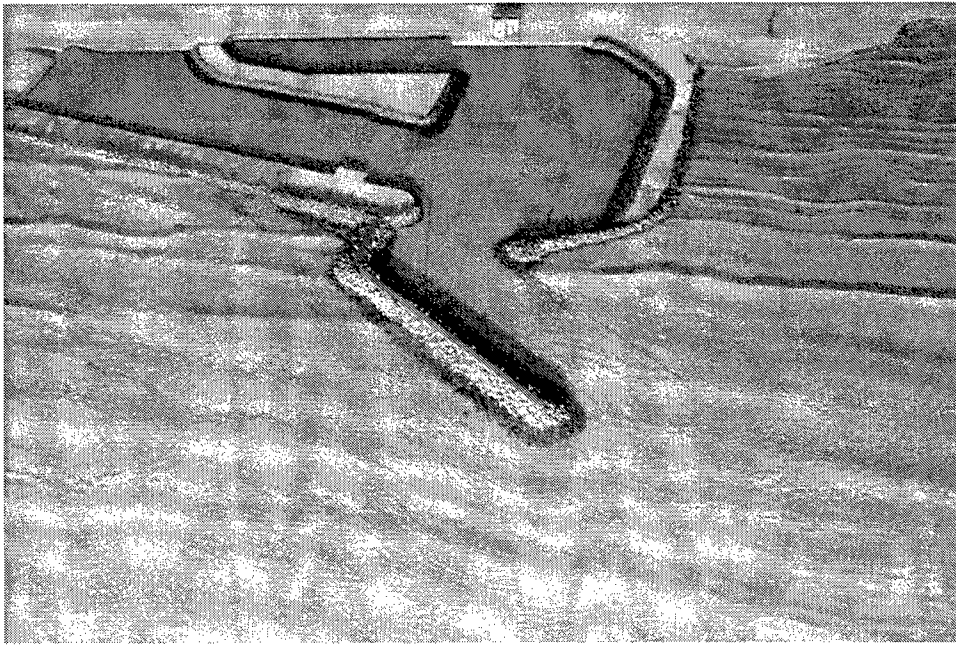
Photo 37. Typical wave patterns for Alternative 2a; 8-sec, 8-ft waves from 180 deg; swl = +1.0 ft mlw
