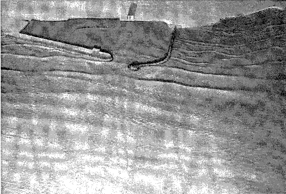
Photo 5. Typical wave patterns for existing conditions; 8-sec, 3-ft waves from 180 deg; swl = +1.0 ft mlw
