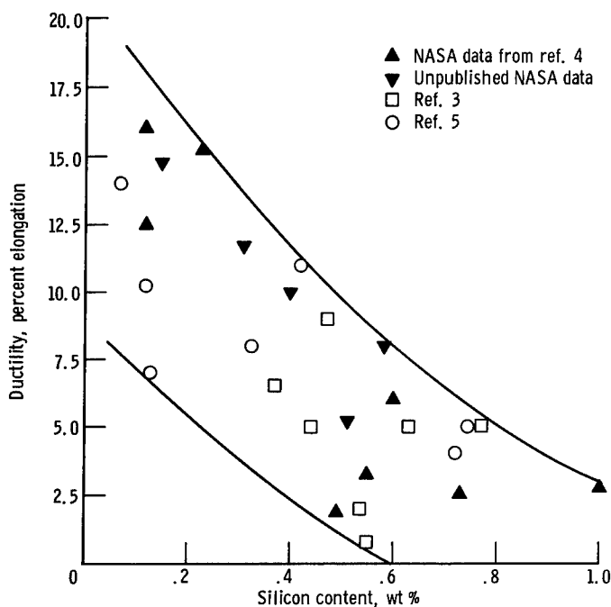
Figure 1. - Compilation of data showing effect of silicon concentration on ductility of L-605 aged 1000 hours at 871 o C.
