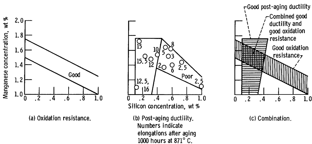
Figure 14. - Combination of good oxidation resistance and good post-aging ductility as function of silicon and manganese concentration. Best combination of properties occurs in range of 0.1- to 0.4-weight-percent silicon and 1.4- to 1.65-weight-percent manganese.
