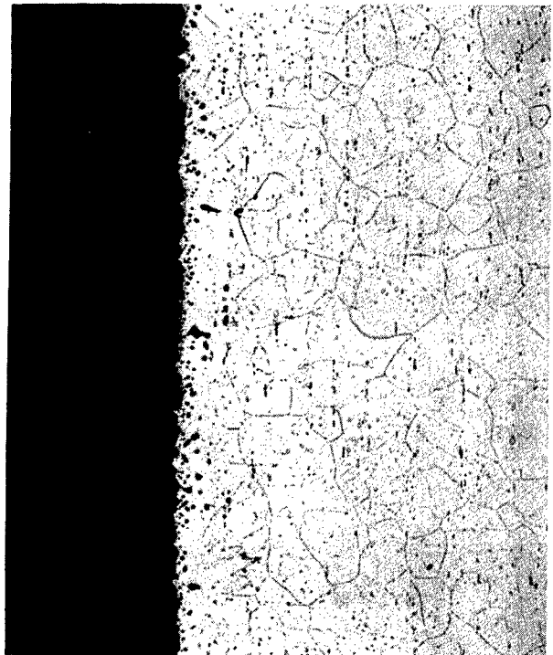
(b) 0.23-weight-percent silicon; 1.52-weight-percent manganese.
