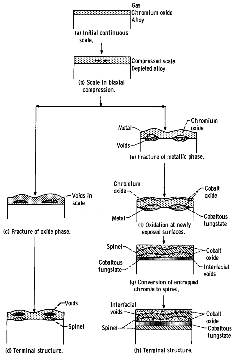
Figure 22. - Schematic representation of course of oxidation of L-605 showing two possible stress-relief modes. Center and left column - oxide fracture associated with smooth, nearly parabolic scale growth; center and right column - alloy fracture associated with anomalous weight increment.
