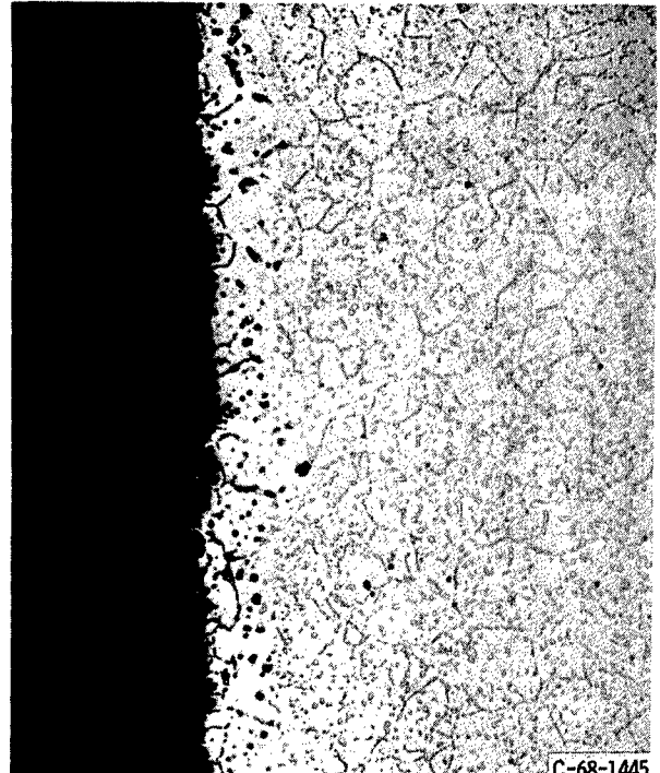
(d) 1.00-weight-percent silicon; 1.11-weight-percent manganese.
