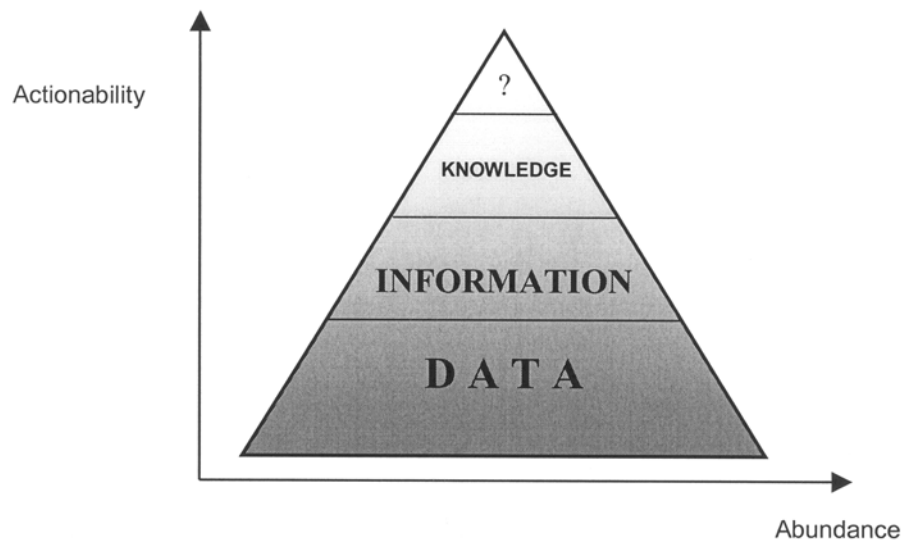
Figure 1. Knowledge Hierarchy
