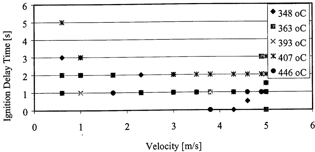
Figure 8 Ignition Delay Time as a Function of Velocity at Different Temperatures for a step height of 57 mm.
