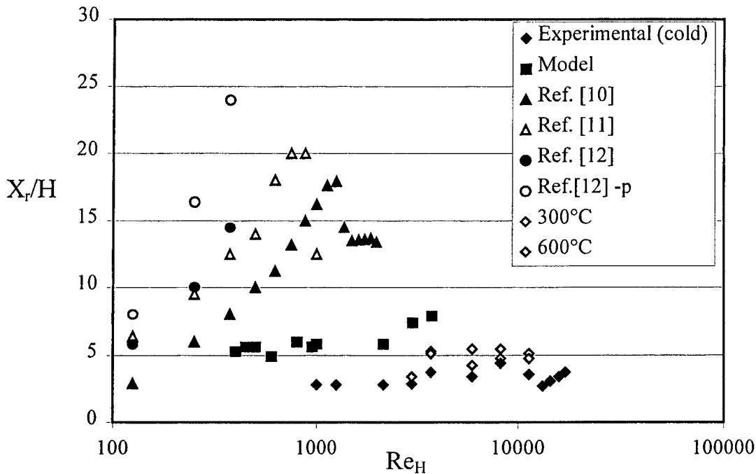
Figure 12 Normalized re-circulation zone length scale as a function of Re_H .
