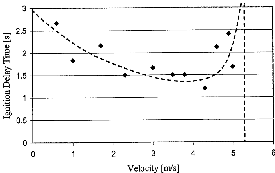
Figure 9 Average Ignition Delay Time as a Function of Velocity
