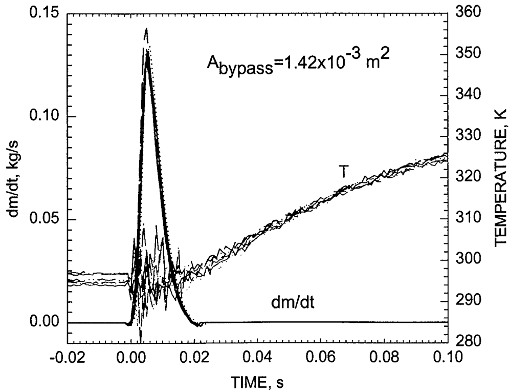
Figure 21. Discharge chamber thermocouple temperature and estimated mass flow of SPGG effluent added to air stream for multiple identical runs.
