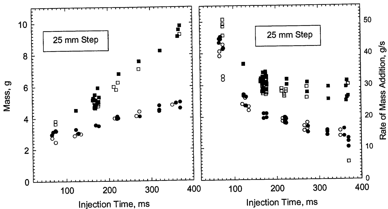
Figure 15. Mass and rate of nitrogen addition required to extinguish high flow (squares) and low flow (circles) air/propane flames: filled symbols, extinction; open symbols, no extinction.
