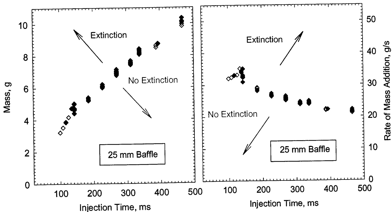
Figure 14. Mass and rate of nitrogen addition required to extinguish 3.88 m/s air flow, 45 mL/s propane flame: filled diamonds, extinction; open diamonds, no extinction.
