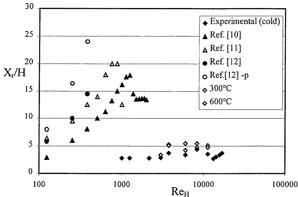
Figure 4 – Evolution of X_r/H as a function of Re_H .
