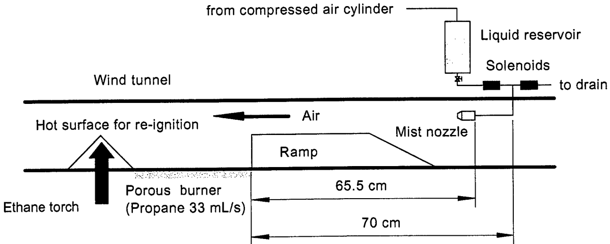
Figure 6. Liquid aerosol agent injection system.
