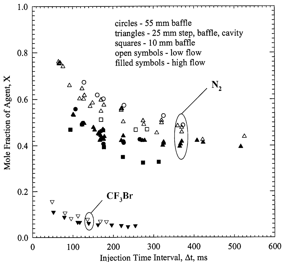
Figure 19. Mole fraction of agents ( N_2 and CF_3Br ) added to air at extinction boundary for high and low flow conditions, as a function of the injection time interval and obstacle geometry.
