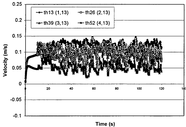
Figure 14 – Time evolution of the velocity for Re=600 measured at x=0.914 m
