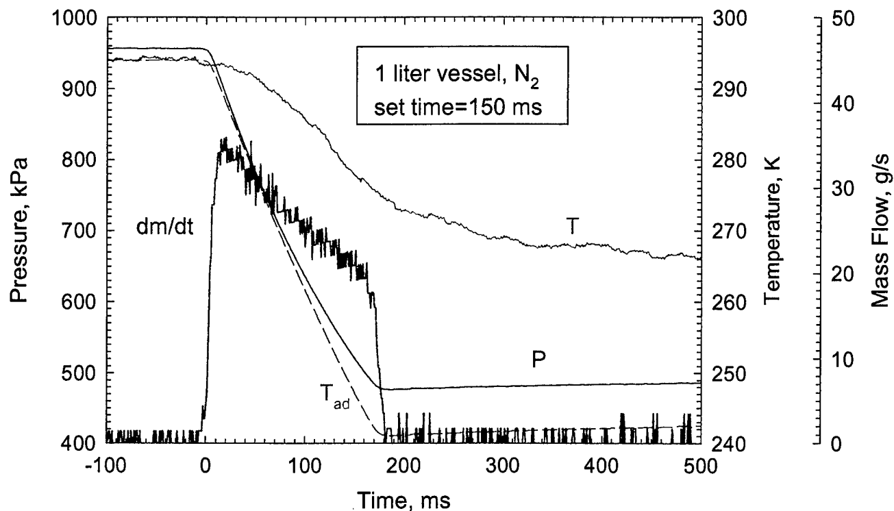
Figure 5. Storage vessel pressure trace and temperature during discharge of nitrogen into TARPF.
