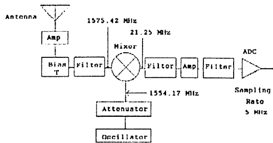
Fig. 3 The modular diagram of the GPS receiver.
