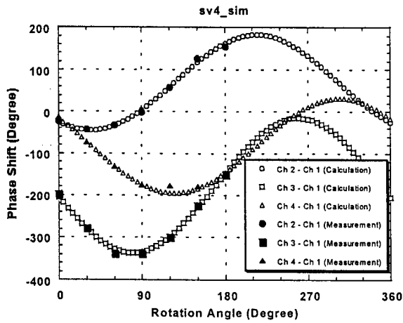
Fig. 8 The phase shift vs. rotation angle measured from the real GPS signal of satellite #4.
