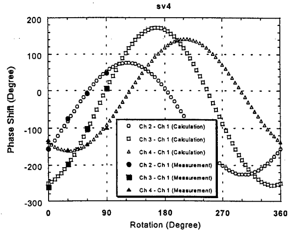
Fig. 10 The phase shift vs. rotation angle measured from the real GPS signal of satellite #4.
