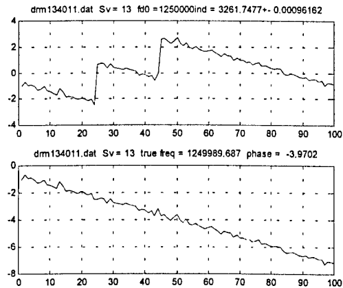
Fig. 4 A typical phase vs. time (in mini-second) results from the GPS acquisition algorithm.
