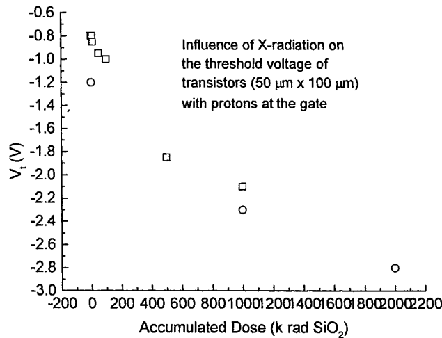
Figure 4. Radiation induced threshold voltage shift in protonated MOSFETs (40 nm gate oxide, 50 μm x 100 μm) due to positive fixed oxide charge generation.
