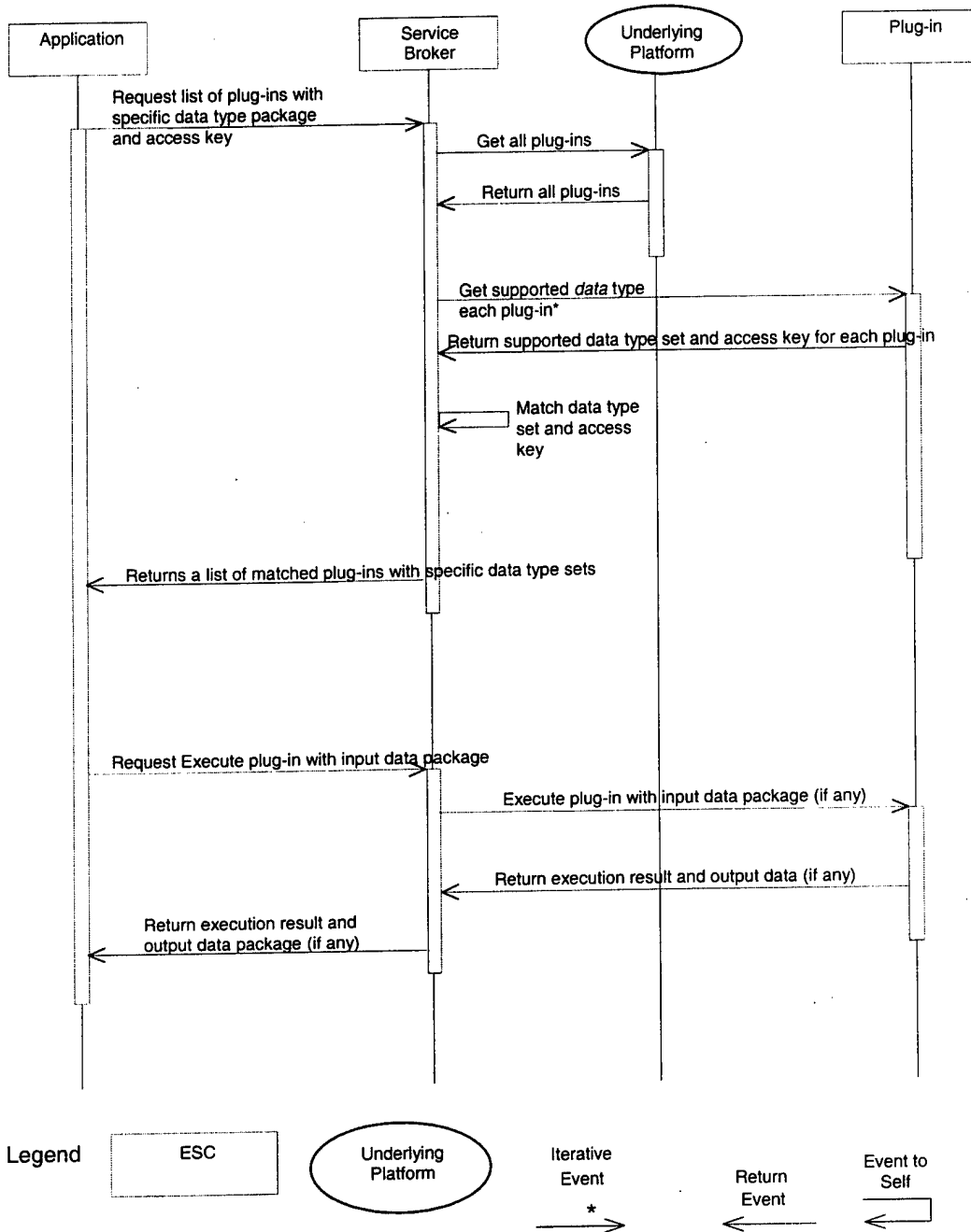
Figure 3: Sequence of Events Among ESCs and the Underlying Platform
