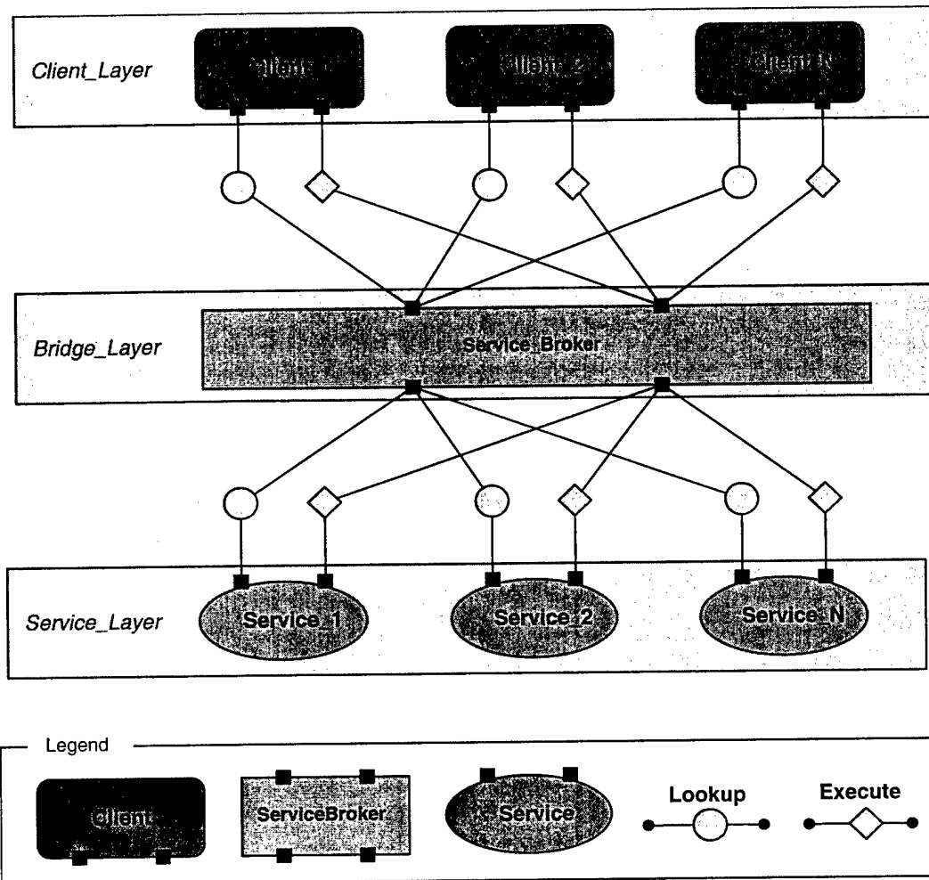
Figure 1: Relationship Among the Three Layers of PAMD
