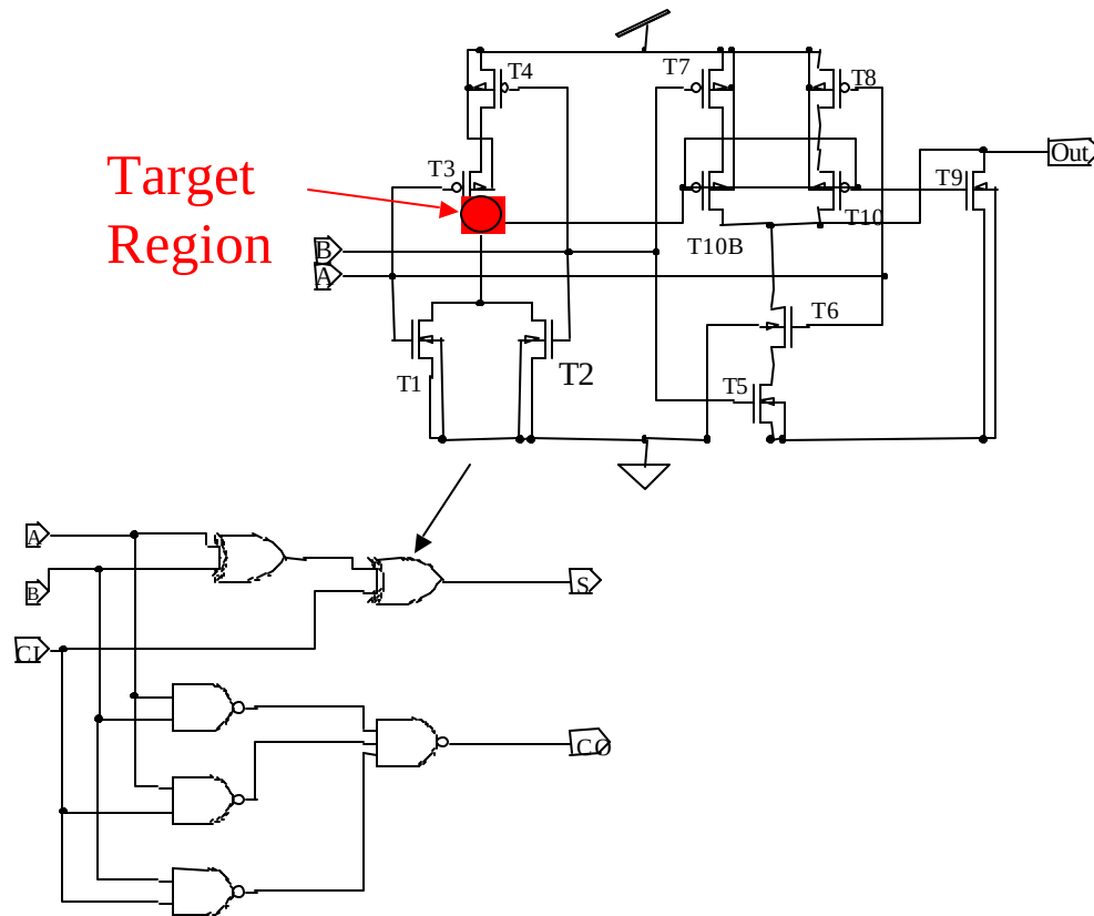
Figure 37. Target Region of Full Adder – Schematic (after [46])
