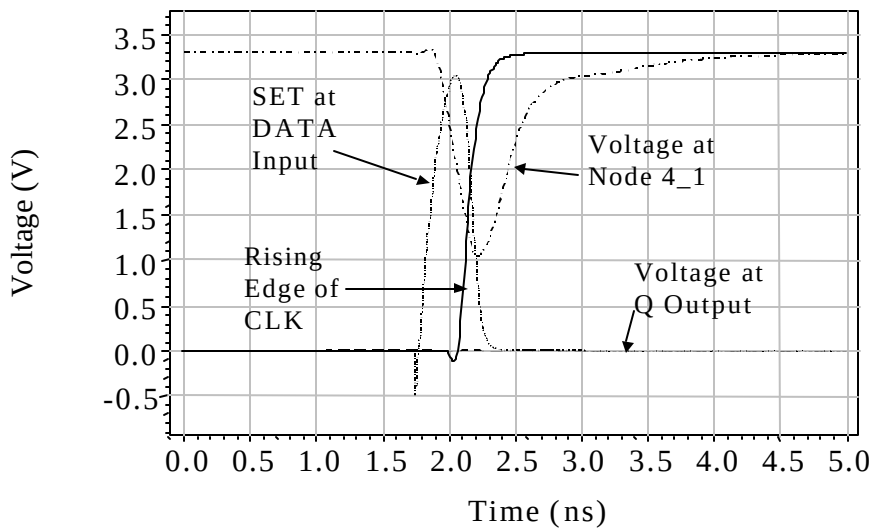
Figure 24. SET Below Latching Threshold
