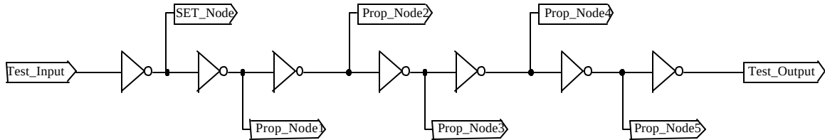
Figure 18. Inverter Propagation Circuit
