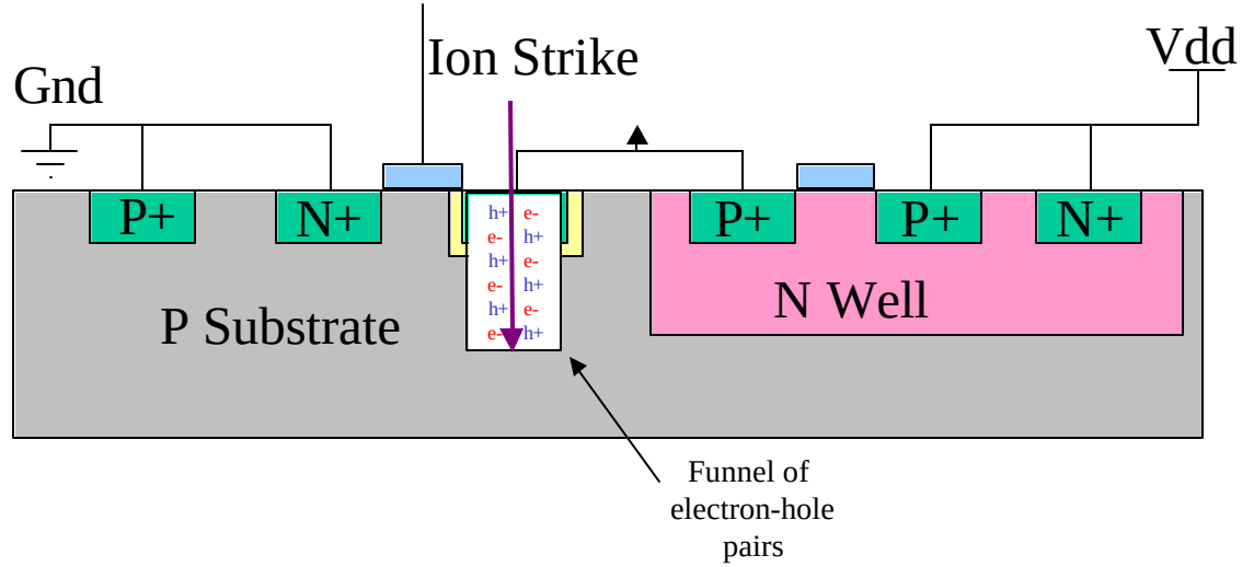
Figure 4. Charge Generation
