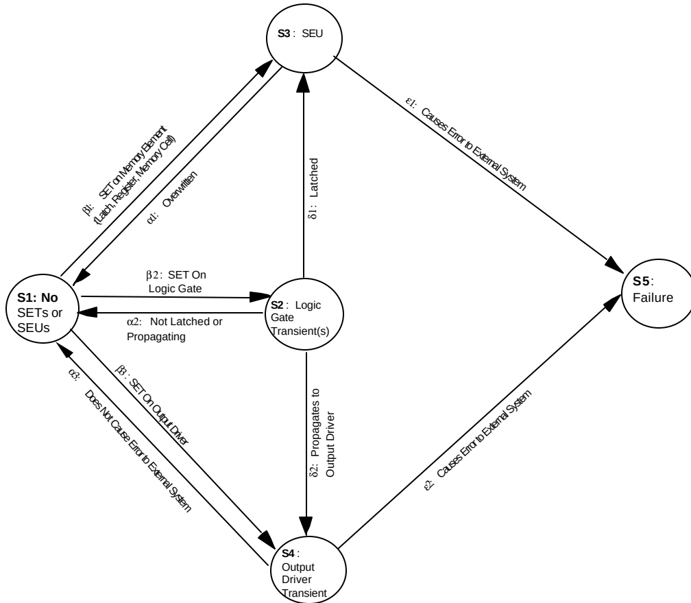
Figure 2. SET-state-transition Model
