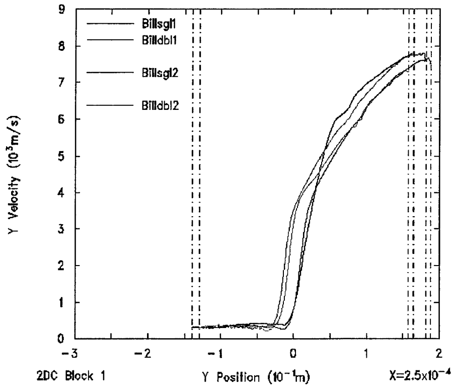
Figure 15. Comparison of reduced mass series 2 jet velocity with full-size counterparts.
