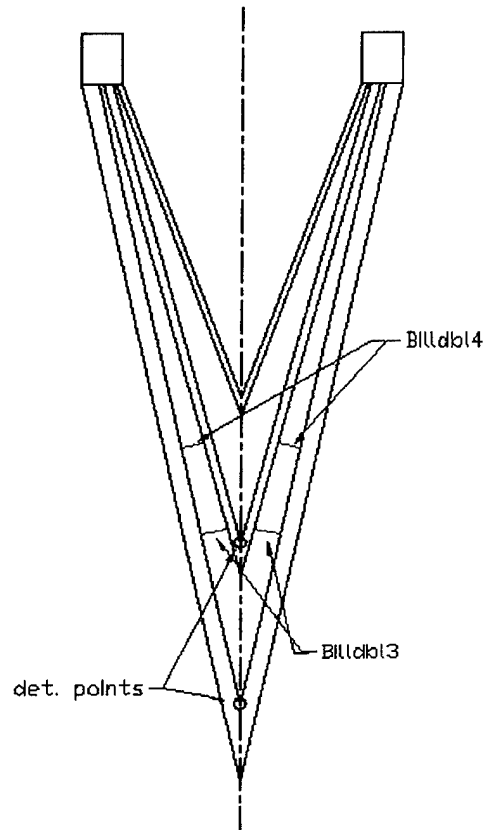
Figure 12. Detonation wave location at the time of inner explosive initiation for Billdbl3 and Billdbl4 simulations.
