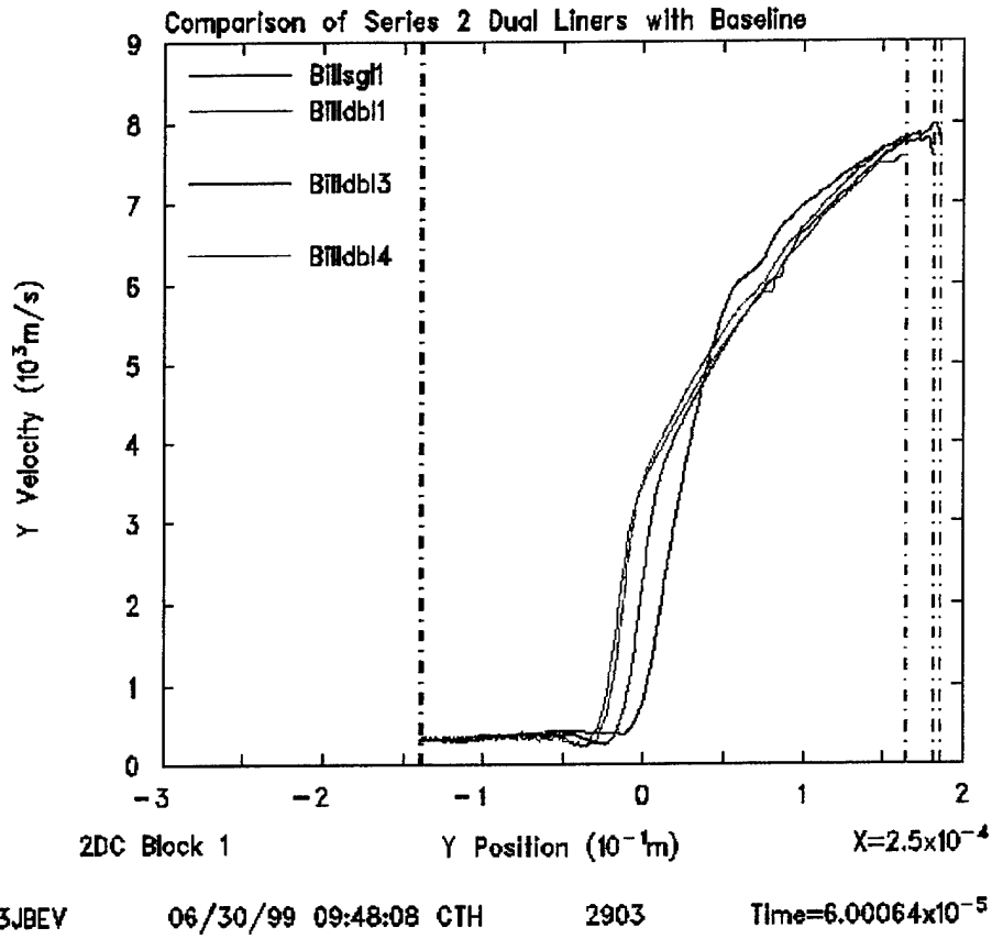
Figure 14. Comparison of series 2 dual confinement simulations sharing a common baseline with the baseline (Billsg11).
