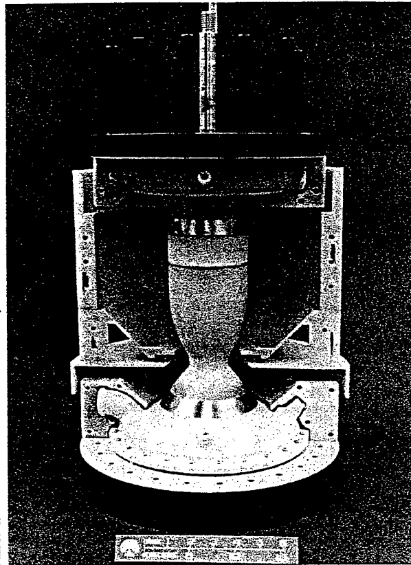
Figure 2: Polycarbonate Plating Development Model and Shielding Shown Ready for Electrodeposition of High Strength Nickel/Cobalt Alloy Produced by the Selective Laser Sintering Process (SLS).
