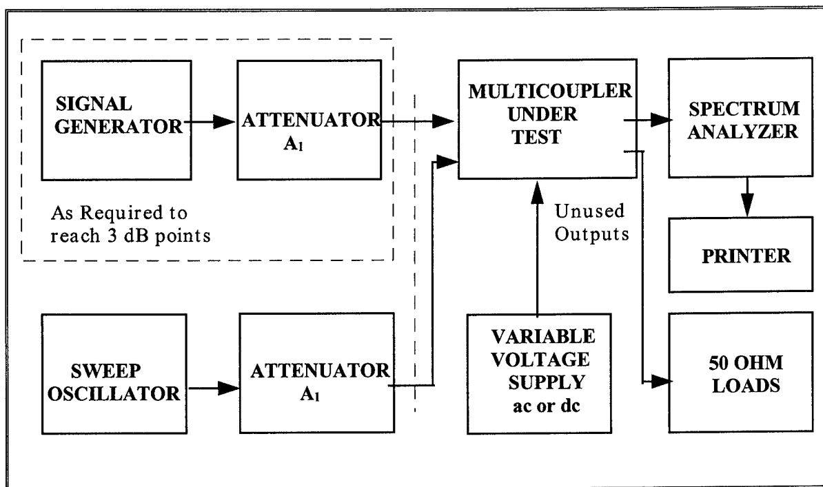
Figure 3-3. Test setup for measurement of bandwidth and small signal power gain (see test 3.2).
