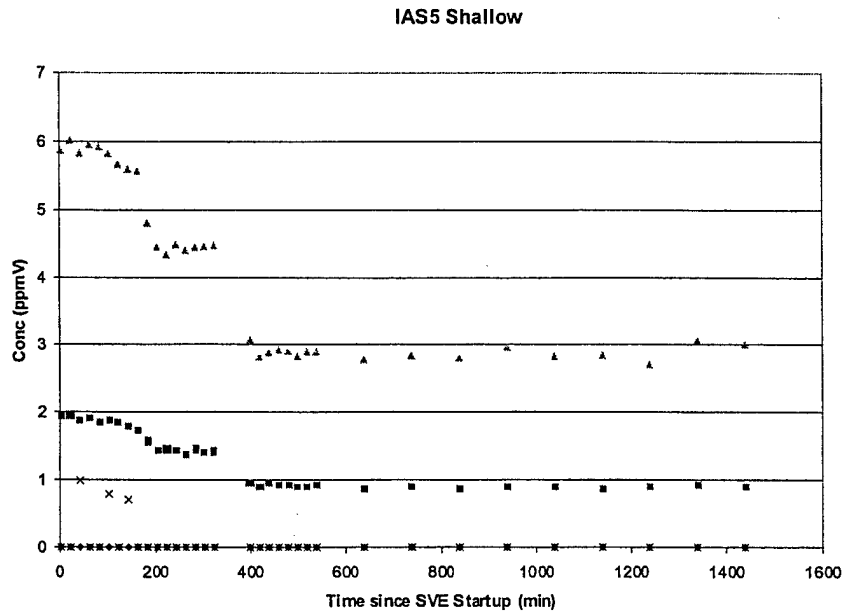
Figure 5. Hydrocarbon off-gas data (ppmv) during the: a) shallow IAS well at 5 ft 3 /min; and 2) deep IAS well at 10 ft 3 /min.
