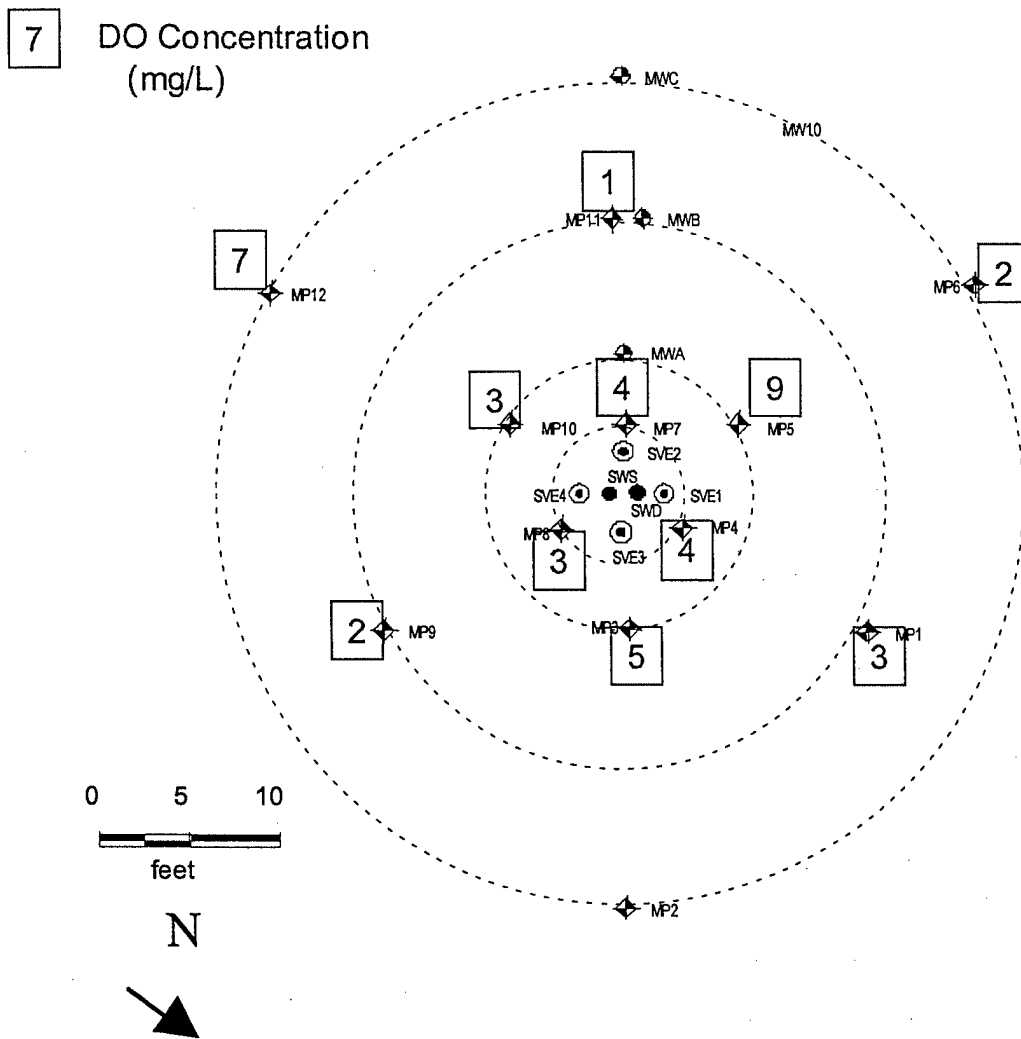
Figure 6. Eielson AFB plan view site map showing dissolved oxygen data taken at the conclusion of the IAS pilot test.
