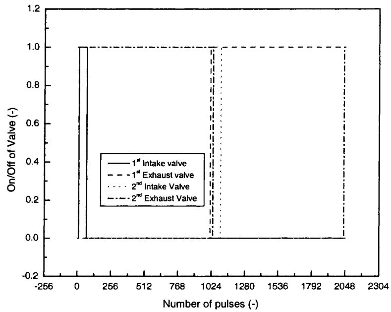
Timing table for the solenoid valves to control the expansion process.
