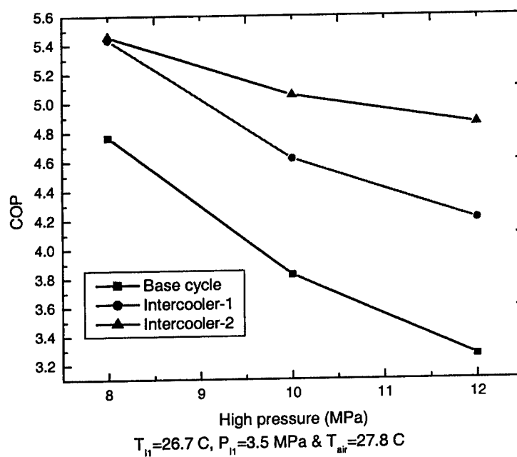
Figure 4.10: Comparison of COPs of transcritical \text{CO}_2 cycles for T_H=26.7^\circ\text{C} and T_{air}=27.8^\circ\text{C} .
