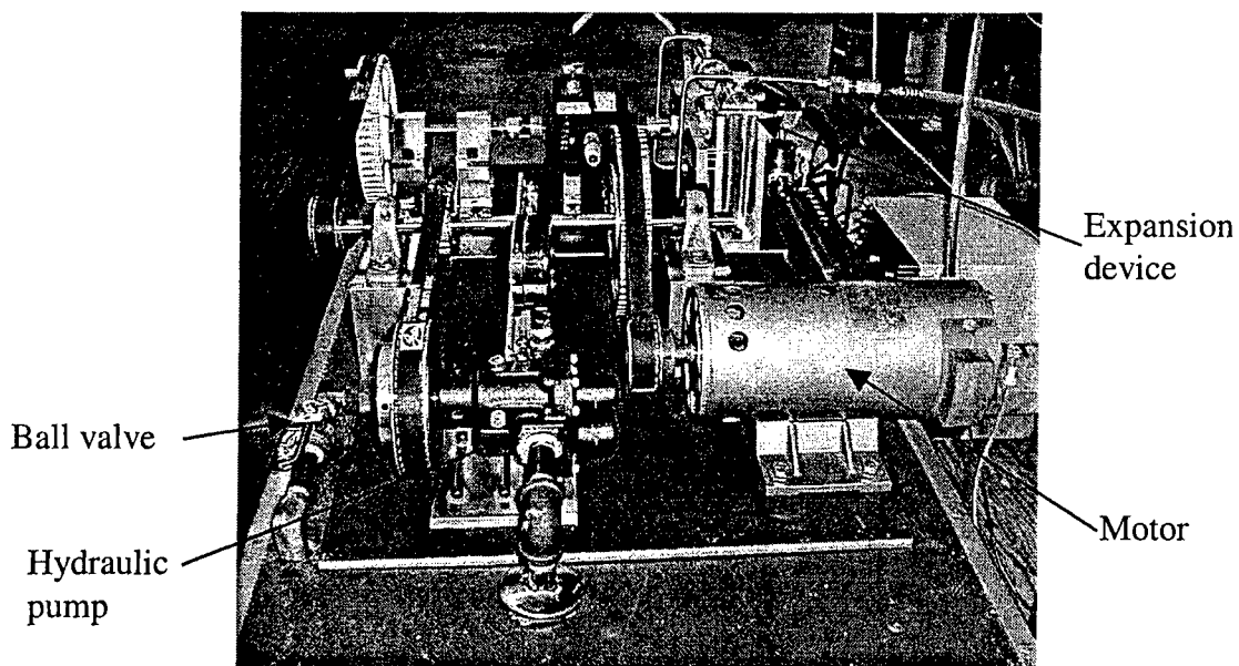
Figure 3.13: Front and side views of the expansion device and hydraulic pump.
