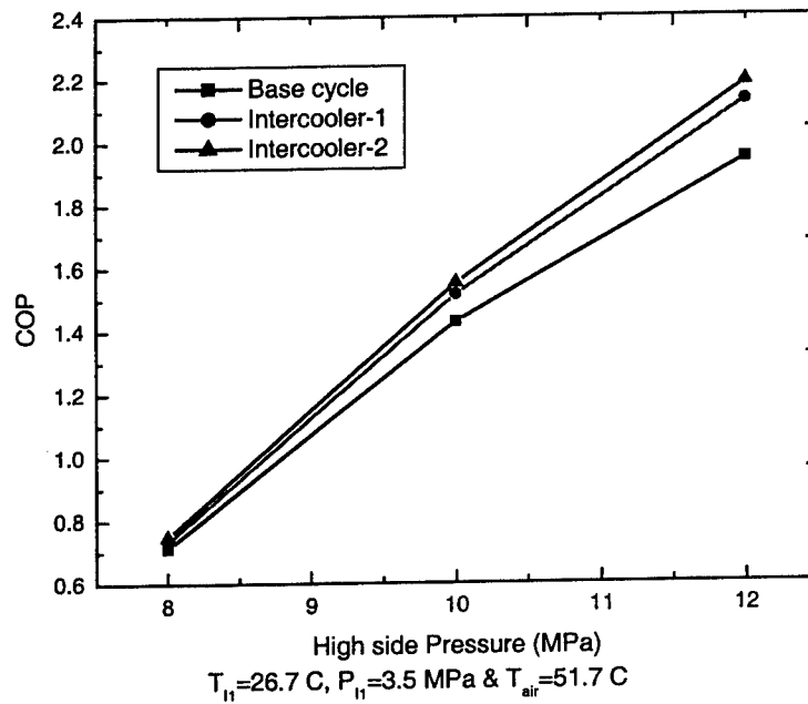
Figure 4.14: Comparison of COPs of transcritical CO 2 cycles for T_H = 26.7^\circ\text{C} and T_{air} = 51.7^\circ\text{C} .
