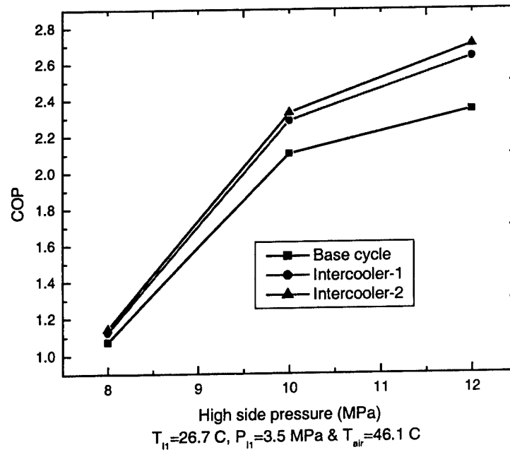
Figure 4.13: Comparison of COPs of transcritical CO 2 cycles for T_H = 26.7^\circ\text{C} and T_{air} = 46.1^\circ\text{C} .
