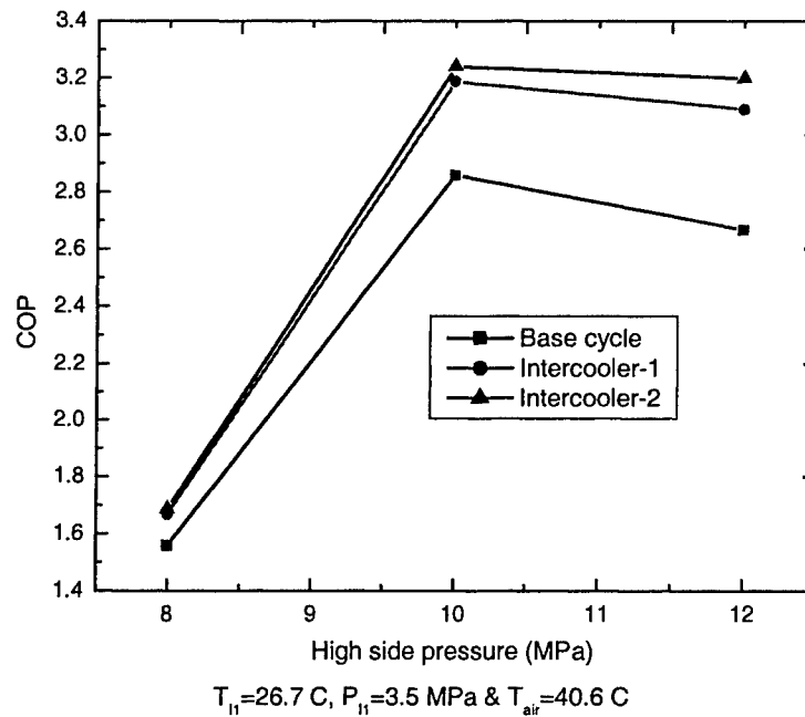
Figure 4.12: Comparison of COPs of transcritical \text{CO}_2 cycles for T_{H1}=26.7^\circ\text{C} and T_{air} = 40.6^\circ\text{C} .
