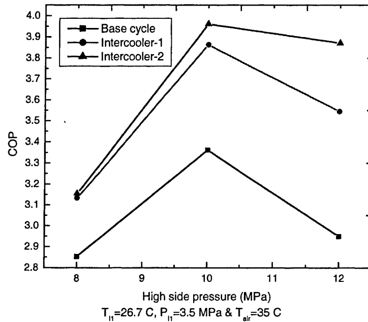
Figure 4.11: Comparison of COPs of transcritical \text{CO}_2 cycles for T_{H1}=26.7^\circ\text{C} and T_{air} = 35.0^\circ\text{C} .
