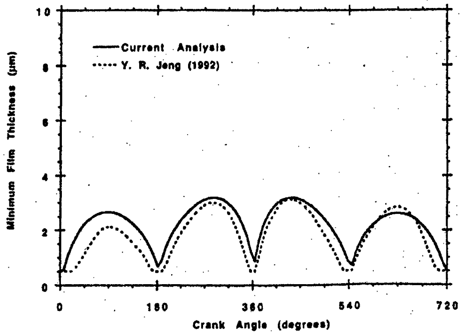
Figure 2.27: Minimum film thickness predicted by models of Jeng and Radkovic and Khonsari [Radkovic and Khonsari, 1997].
