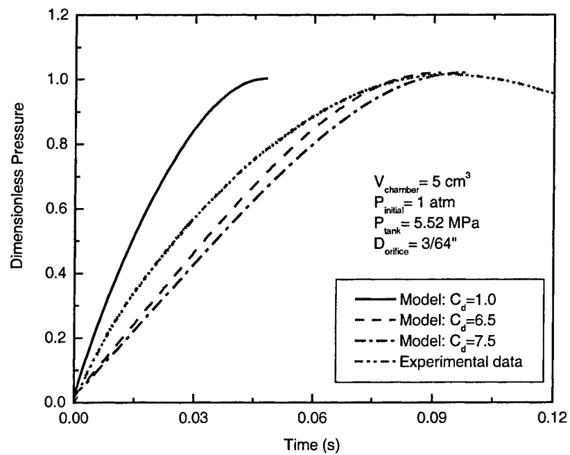
Figure 2.22: Determination of discharge coefficient for sudden contraction.
