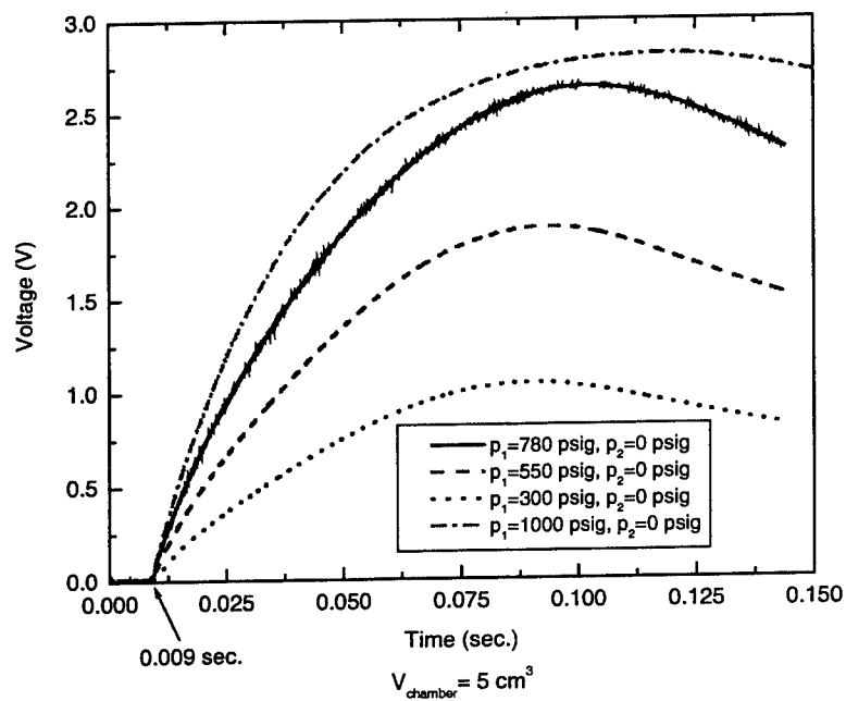
Figure 3.2: Filling behaviors of CO 2 in the chamber with the intake valve ( D_{\text{orifice}} = 3/64 \text{ in.} ).
