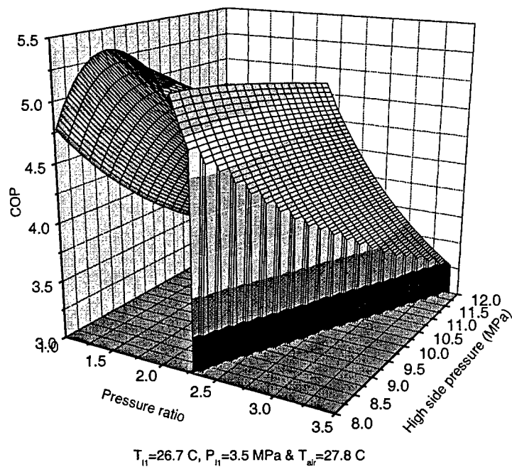
Figure 4.20: Behavior of COP of Intercooler cycle for T_{H1}=26.7^\circ\text{C} and T_{air}=27.8^\circ\text{C} .
