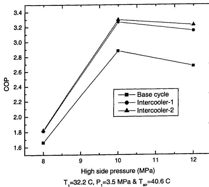
Figure 4.17: Comparison of COPs of transcritical \text{CO}_2 cycles for T_{H1}=32.2^\circ\text{C} and T_{air}=40.6^\circ\text{C} .
