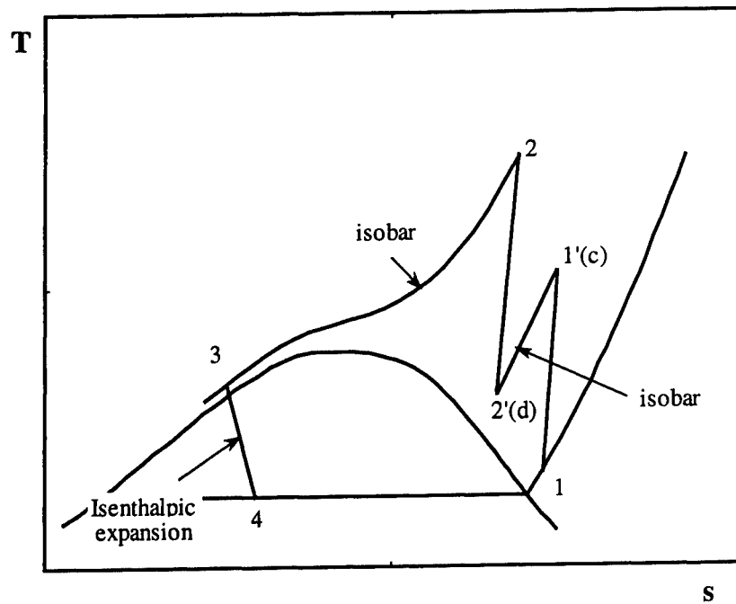
Figure 1.11: Temperature-entropy diagram of transcritical CO 2 cycle with two-stage compression with intercooling.
