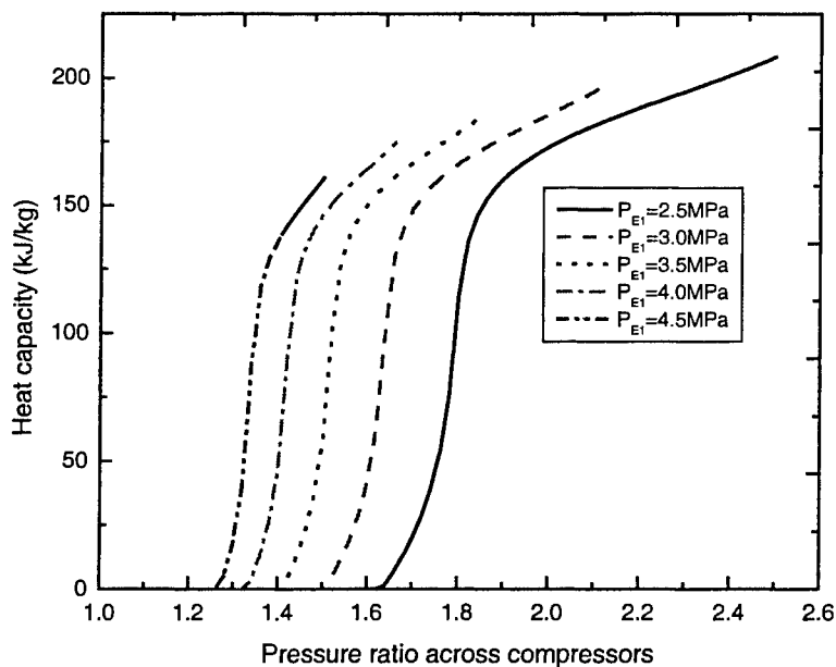
Figure 4.8: Effect of pressure at the inlet to the evaporator on heat removal capacity of Economizer cycle.
