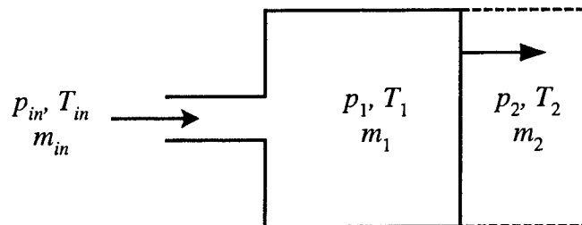
Figure 2.31: Intake process.
