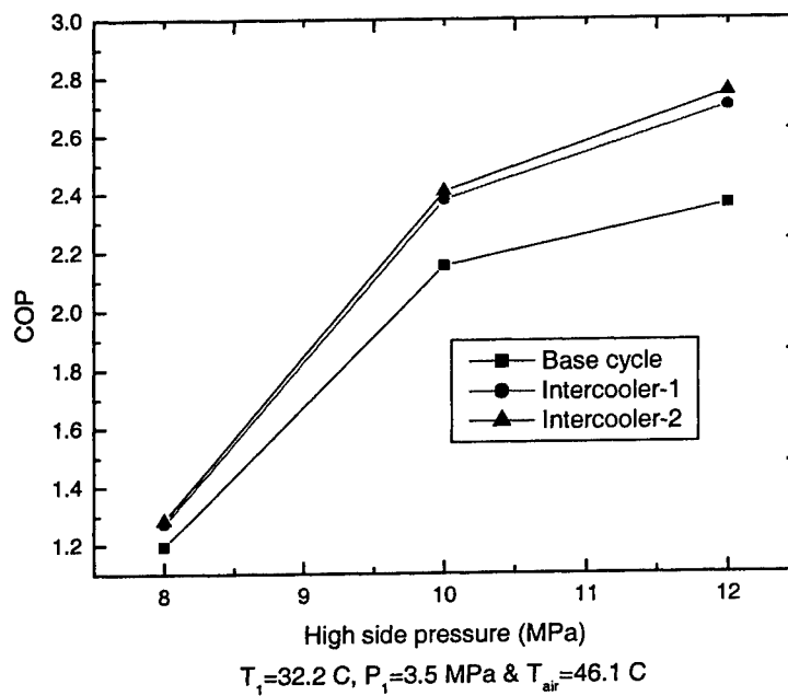
Figure 4.18: Comparison of COPs of transcritical \text{CO}_2 cycles for T_{H1}=32.2^\circ\text{C} and T_{air}=46.1^\circ\text{C} .
