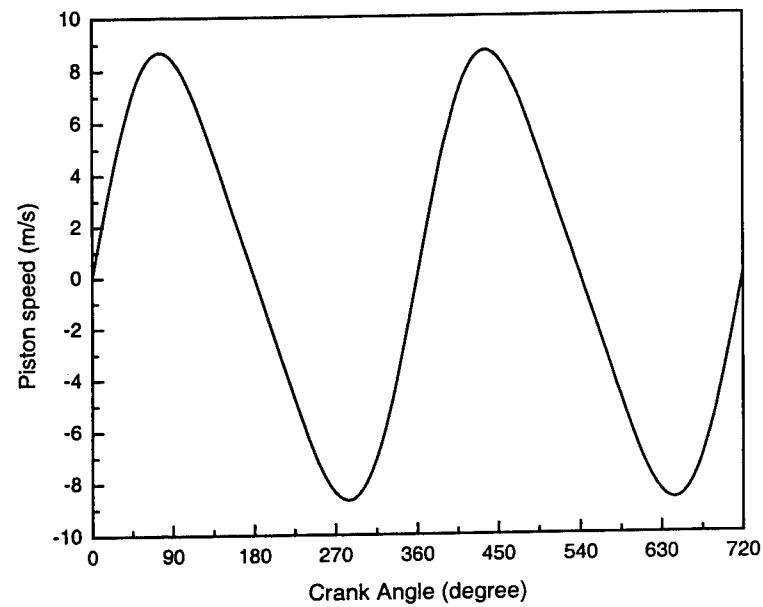
Figure 2.25: Piston speed versus crank angle for 2000 rpm engine speed.
