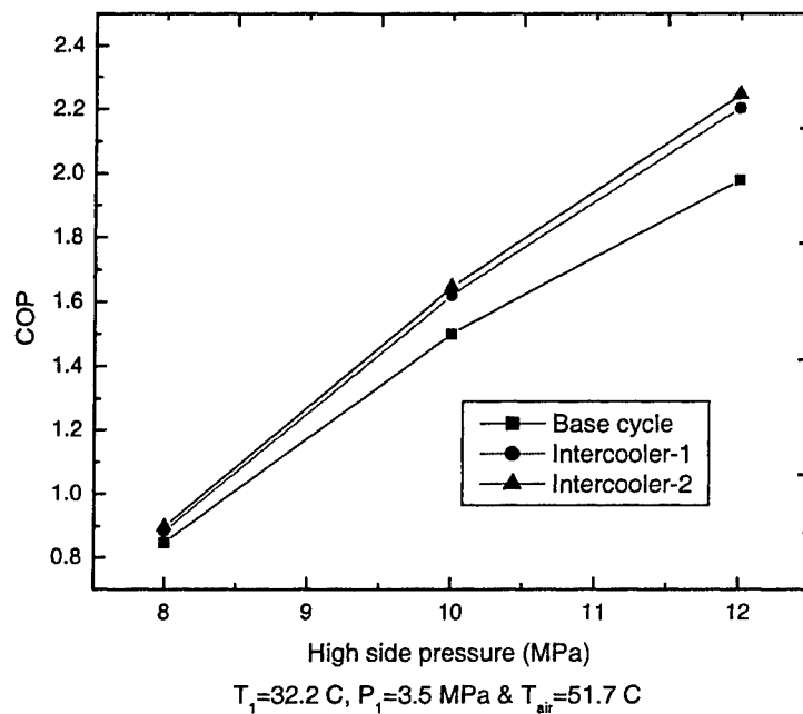
Figure 4.19: Comparison of COPs of transcritical \text{CO}_2 cycles for T_{H1}=32.2^\circ\text{C} and T_{air}=51.7^\circ\text{C} .
