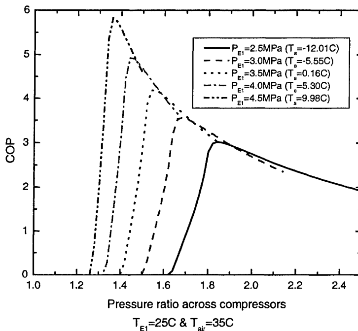
Figure 4.7: Effect of pressure at the inlet to the evaporator on COP of Economizer cycle.
