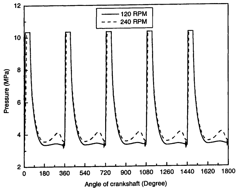
Figure 4.26: Repeat of the same trends of the pressure behavior for 120RPM and 240RPM.
