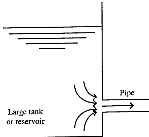
Figure 2.12: Entrance loss.
