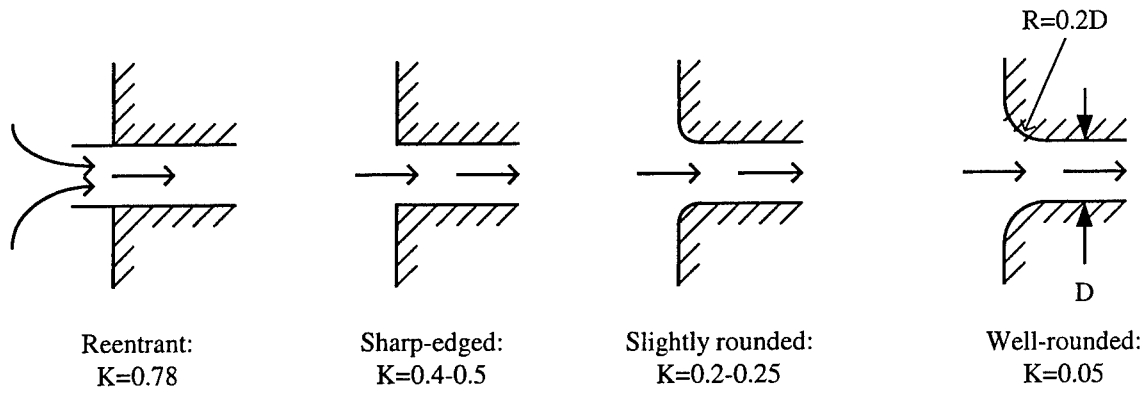
Figure 2.13: Entrance loss coefficients [Evet and Liu, 1987].
