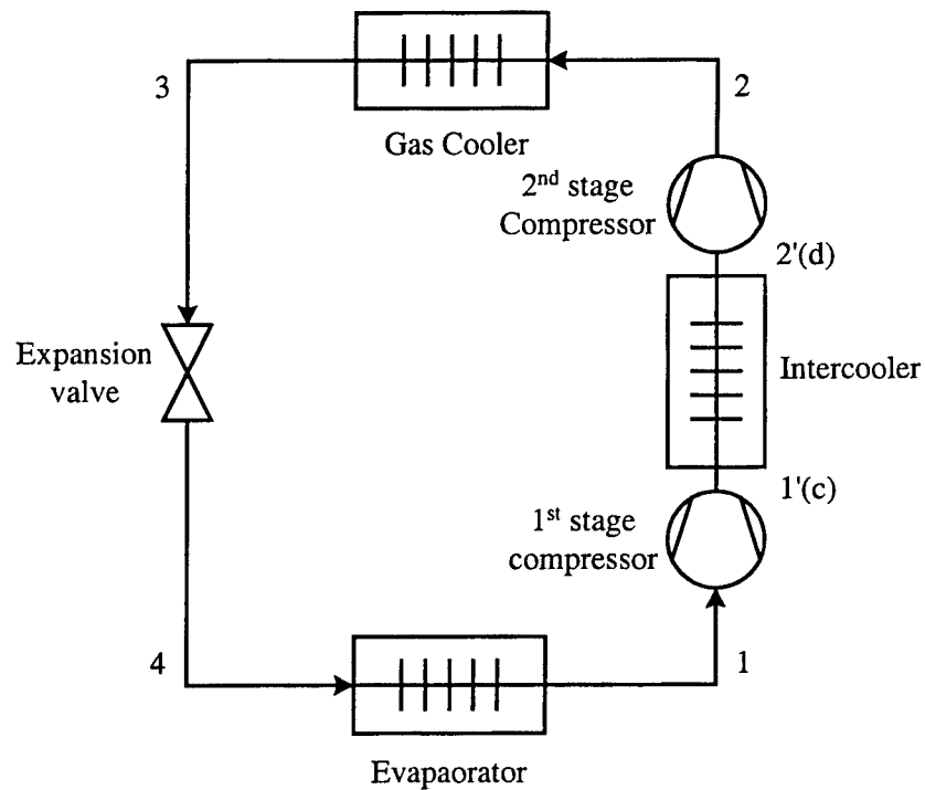
Figure 1.10: Schematic of transcritical CO 2 cycle with two-stage compression with intercooling.
