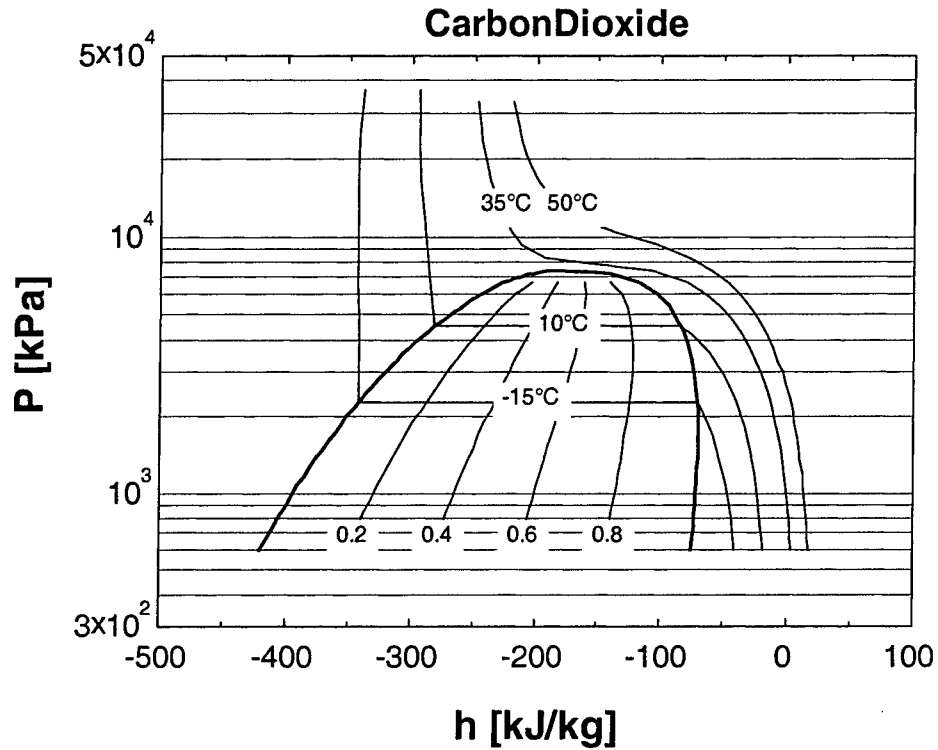
Figure 4.15: Thermodynamic characteristics of CO 2 on P-h diagram.
