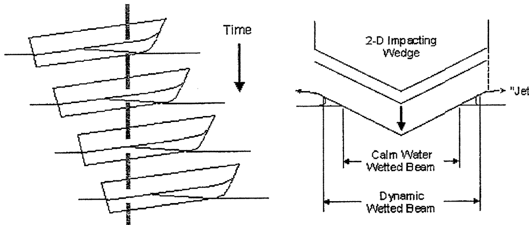
Figure 15. Impacting Wedges [1]
