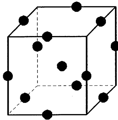
Figure 18. Box-Behnken Design
