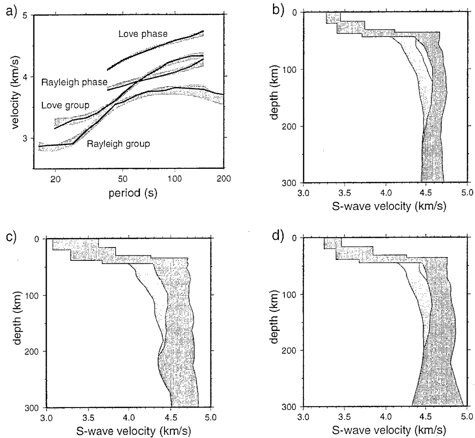
Figure 8: Observed dispersion curves and results of inversion for three data sets. (a) Observed dispersion curves at a point in Iran ( 30^{\circ}\text{N} , 60^{\circ}\text{E} ). The black lines are observations derived from the dispersion maps and the grey shaded zones represent the range of dispersion curves from the ensemble of acceptable models shown in (b). (b) simultaneous inversion of group and phase speeds (CUB2.0), (c) group speed alone, and (d) phase speed alone. The full width of the ensemble of acceptable models is indicated, where v_{sh} is dark grey and v_{sv} is light grey.
