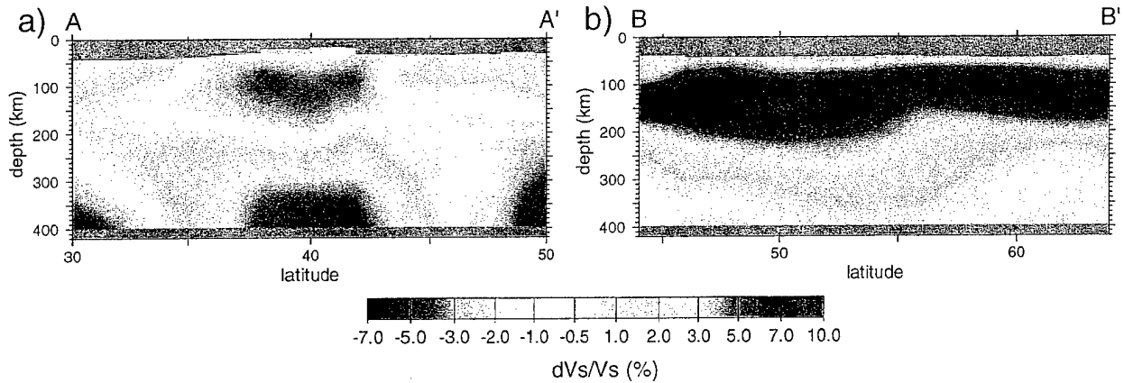
Figure 9: Vertical slices of the v_s model from CUB2.0 plotted as percent deviation from AK135. Locations of the profiles are shown in Figure 1.
