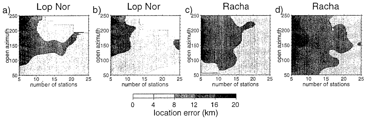
Figure 20: Mislocation using the 3-D model CUB2.0.TH, presented as a function of number of stations and open azimuth, determined by randomly choosing subsets of the reported travel times for four events: (a) Lop Nor, May 26, 1990; (b) Lop Nor, Sept 25, 1992; (c) Racha, May 3, 1991; (d) Racha, July 4, 1991.
