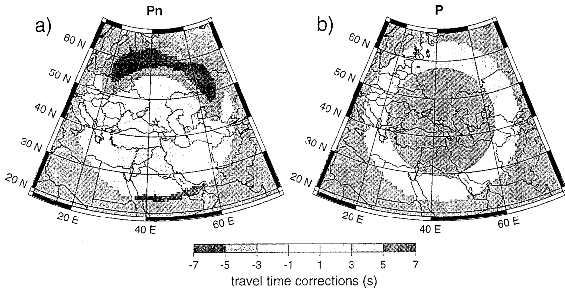
Figure 14: Example of P_n and P travel time correction surfaces computed for a surface source for station KIV. The corrections here are relative to the 1-D model IASP91.
