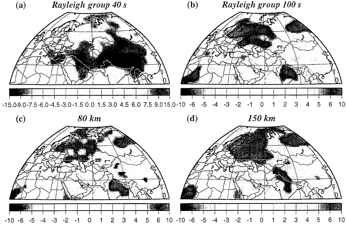
Figure 7: Selected dispersion maps and horizontal slices of the model at the periods and depths indicated.
