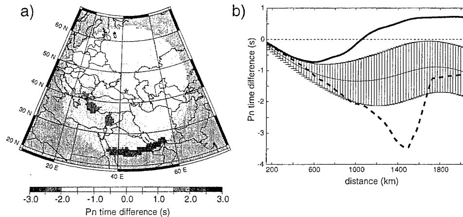
Figure 13: Effect of the v_s to v_p conversion on P_n travel times. (a) Difference between P_n travel times from CUB2.0_TH and CUB2.0_EMP centered on stations KIV (Kislovodsk, Russia). Positive values mean CUB2.0_TH travel times are faster than those from CUB2.0_EMP. (b) Solid line shows the P_n travel time difference for profile B - B' and the dashed line for A - A' from Figures 1 and 9. One standard deviation errors bars show the geographical average across the region of study (Figure 1).
