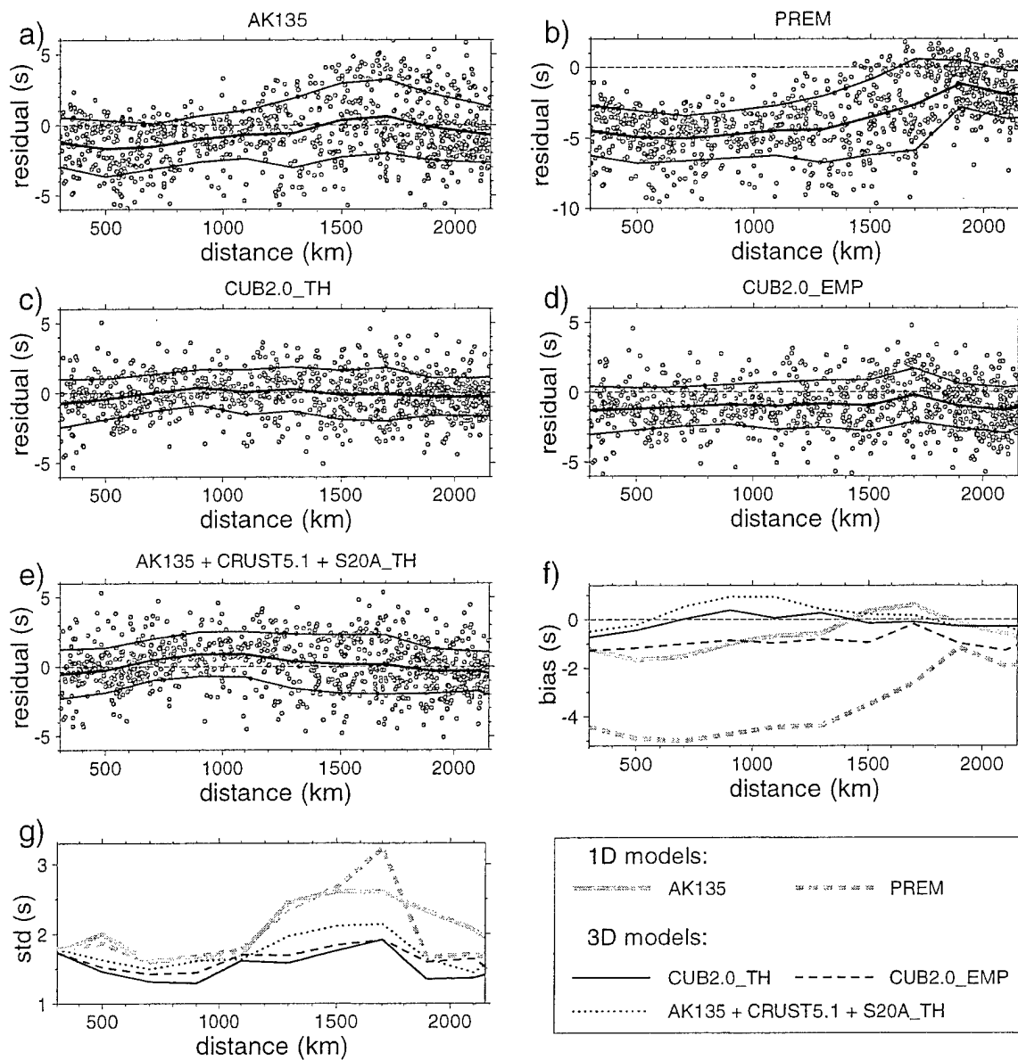
Figure 18: Residuals between the empirical phase path anomalies for P_n and P and predictions. (a)-(e) Residuals from a number of models, plotted versus epicentral distance. Running average (bias) and standard deviation are shown as the black lines. Cluster time baseline shifts have not been applied. (f) - (g) The running residual bias and standard deviation shown for the various models.
