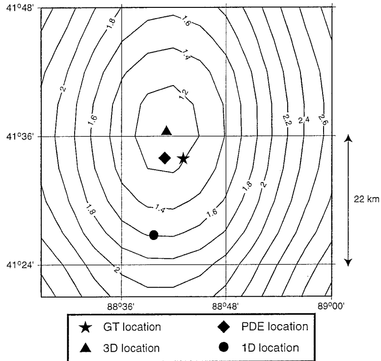
Figure 5: Example of the grid-search location algorithm. Contours of rms-misfit using a 3-D model for a grid of hypothesized epicenters for an explosion at the Lop Nor test site (May 26, 1990; 54 reporting stations). Units are seconds. The GT1-2 location is indicated with a star, the best-fit locations using the 3-D and 1-D models are shown with a triangle and a circle, respectively, and the PDE location is shown with a diamond.
