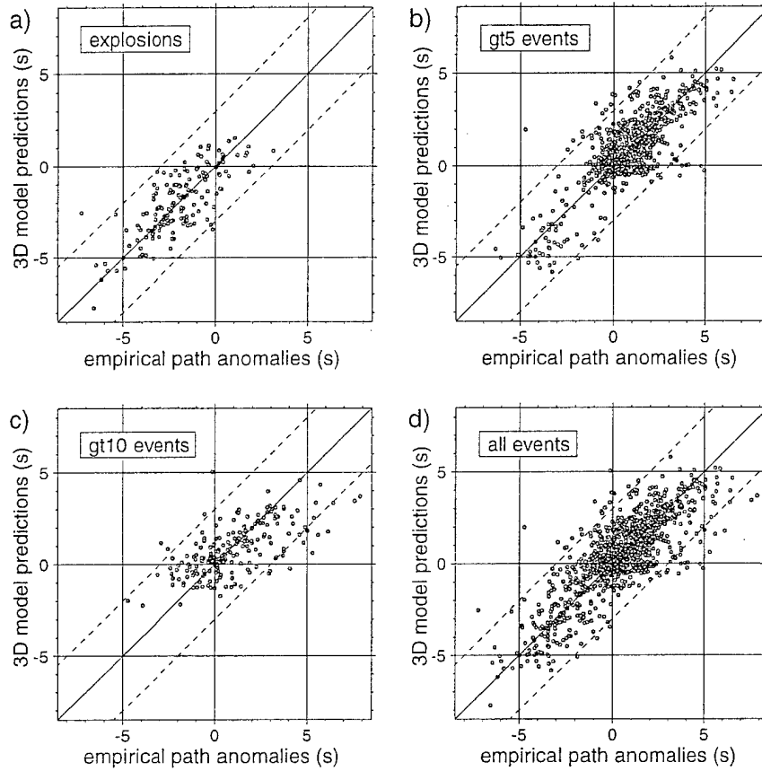
Figure 17: Overall comparison between the P and P_n travel times predicted by the 3-D model CUB2.0_TH and the empirical phase path anomalies. The cluster time baseline shifts listed in Tables 5 - 7. have been applied and misfit statistics are also listed in these tables.
