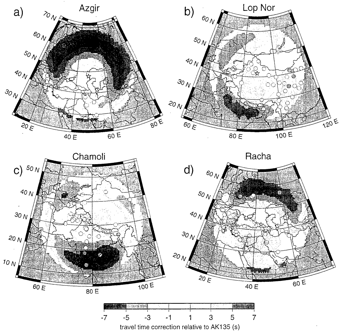
Figure 15: Cluster-centered travel time correction surfaces for four cluster regions. The colored contours are the predictions from the 3-D model CUB2.0_TH referenced to the travel time from the 1-D model AK135. The symbols are the empirical phase path anomalies, color-coded similarly to the model predictions. The cluster time baseline shift is indicated in Tables 5 and 6. (a) and (b) are explosions in the Azgir and Lop Nor clusters and (c) and (d) are earthquakes in the Chamoli and Racha clusters, respectively.
