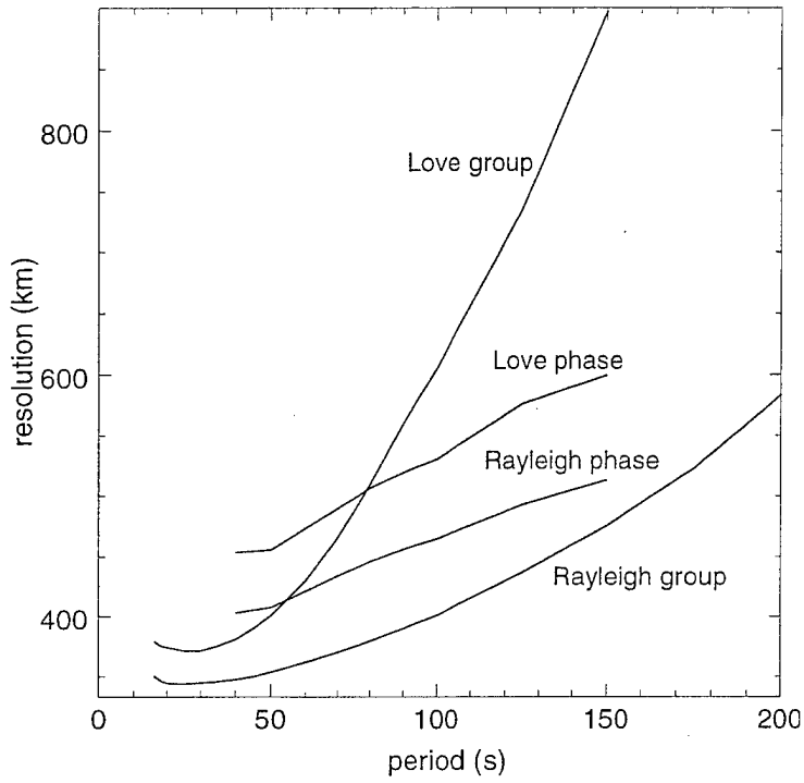
Figure 6: Resolution of the dispersion maps averaged across the region of study.
