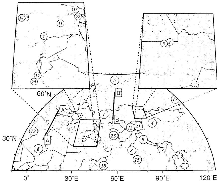
Figure 1: Locations of the explosion and earthquake clusters. Numbers refer to clusters identified in Table 3. Lines A - A' and B - B' refer to the vertical model profiles shown in Figure 9.
