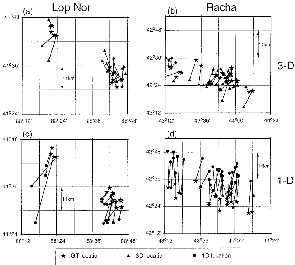
Figure 19: Mislocation vectors for two event clusters for (left column) explosions on the Lop Nor test site and (right column) earthquakes near Racha, Georgia. (a) and (b) 3-D model (CUB2.0.TH) locations. (c) and (d) 1-D model (AK135) locations. Stars mark GT locations, triangles and circles are 3-D and 1-D model locations, respectively.
