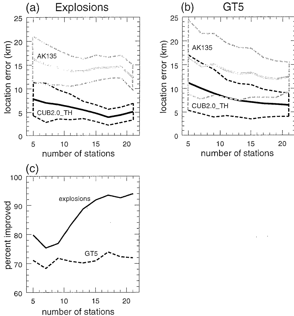
Figure 21: Location error for the 3-D and 1-D models, plotted as a function of the number of reporting stations, determined by randomly choosing subsets of the reported travel times in which open-azimuth is constrained to be less than 180^\circ . (a) and (b) Average (solid lines) and standard deviation (dashed lines) are shown for explosions and GT5 earthquakes for CUB2.0_TH (black lines) and AK135 (grey lines). (c) Percent of the events for which the location error is smaller using the 3-D model than the 1-D model for explosions (solid line) and GT5 earthquakes (dashed line).
