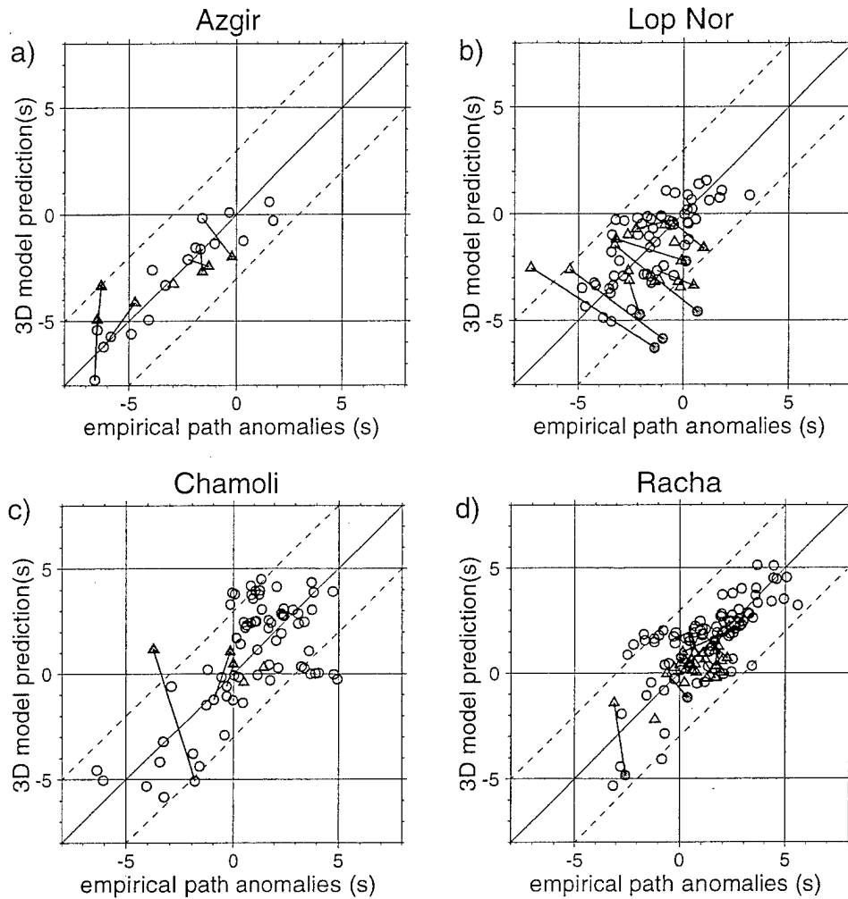
Figure 16: Comparison between the P and P_n travel times predicted by the 3-D model CUB2.0.TH and the empirical phase path anomalies for the four event clusters shown in Figure 15. The empirical path anomalies are on the horizontal axis, paired with the model predictions on the vertical axis. Circles are P_n and triangles are P . Phases have been re-identified using the 3-D model; bars link phases originally identified with the 1-D model AK135 (shaded gray) to the re-identified phases (unshaded). The cluster time baseline shifts listed in Tables 5 and 6 have been applied. The dashed lines mark the location of \pm 3 sec residuals.
