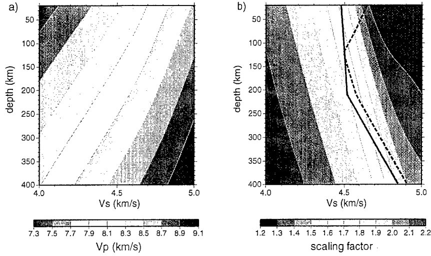
Figure 10: v_p models at the midpoint of two profiles. (a) Grid used for the theoretical v_s to v_p conversion. (b) The theoretical conversion presented as the logarithmic scaling factor d \ln v_s / d \ln v_p . The solid black line is v_s from the 1-D model AK135 and the dashed line is v_s converted from AK135 v_p by the theoretical conversion.
