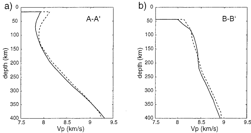
Figure 11: v_p model at the mid-points of profiles (a) A - A' and (b) B - B' from Figures 1 and 9. The solid line represents the theoretical conversion from v_s (i.e., CUB2.0_TH) and the dashed line is from the empirical scaling relation d \ln v_s / d \ln v_p = 2.0 in which AK135 is used as the reference (i.e., CUB2.0_EMP).
