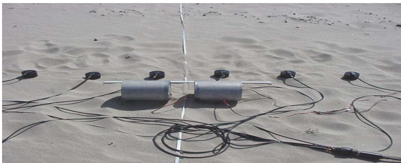
Figure 27. Seismometer array and tube surface sources
