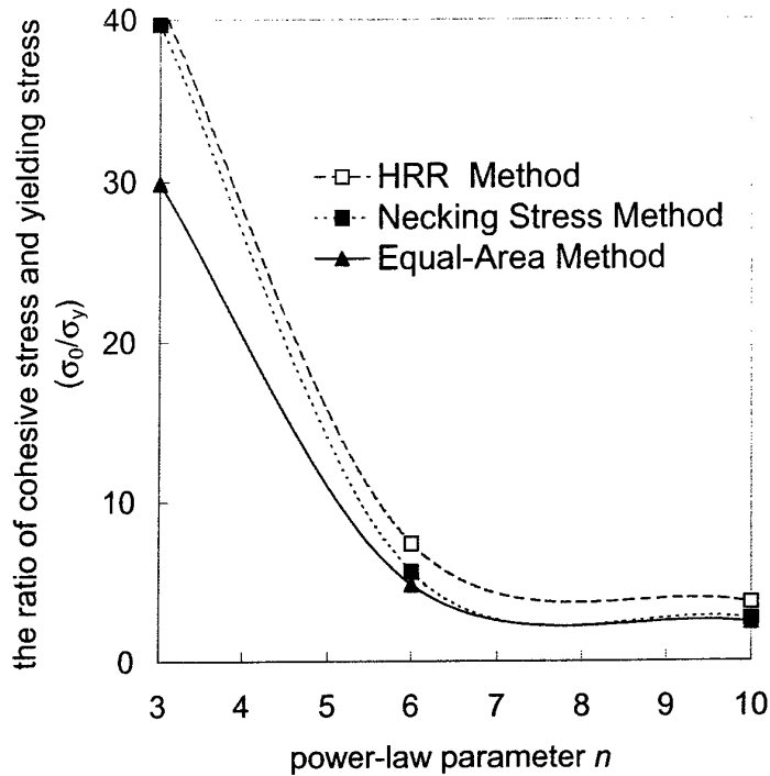
Figure 7 A comparison of cohesive stress by using the HRR Method, Necking Stress Method and Equal-Area Method.
