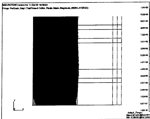
Figure 3 Plastic deformations under plane strain conditions: (a) front face yielding, (b) break-through, and (c) cross-section yielding
