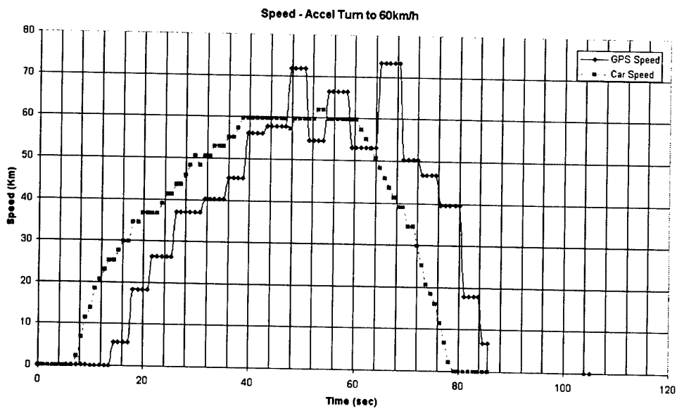
Figure 36: Speed plot for Accelerated Turn to 60 km/hr
