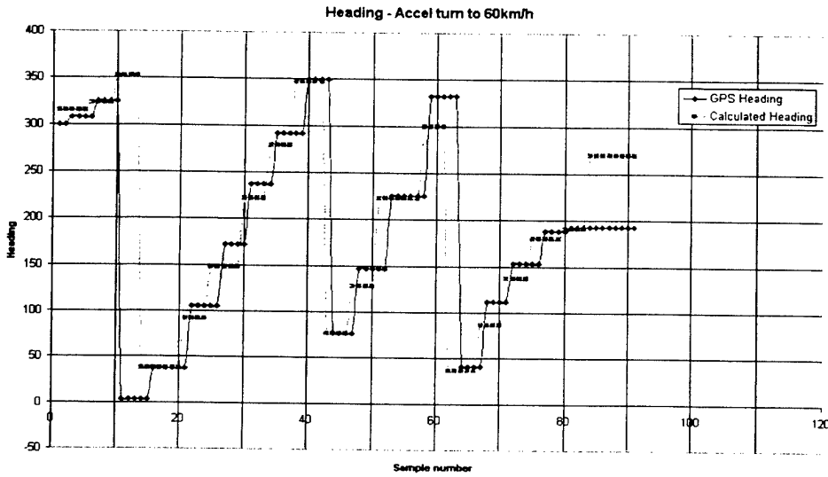
Figure 18: Heading Plot for Accelerated Turn to 60 km/hr
