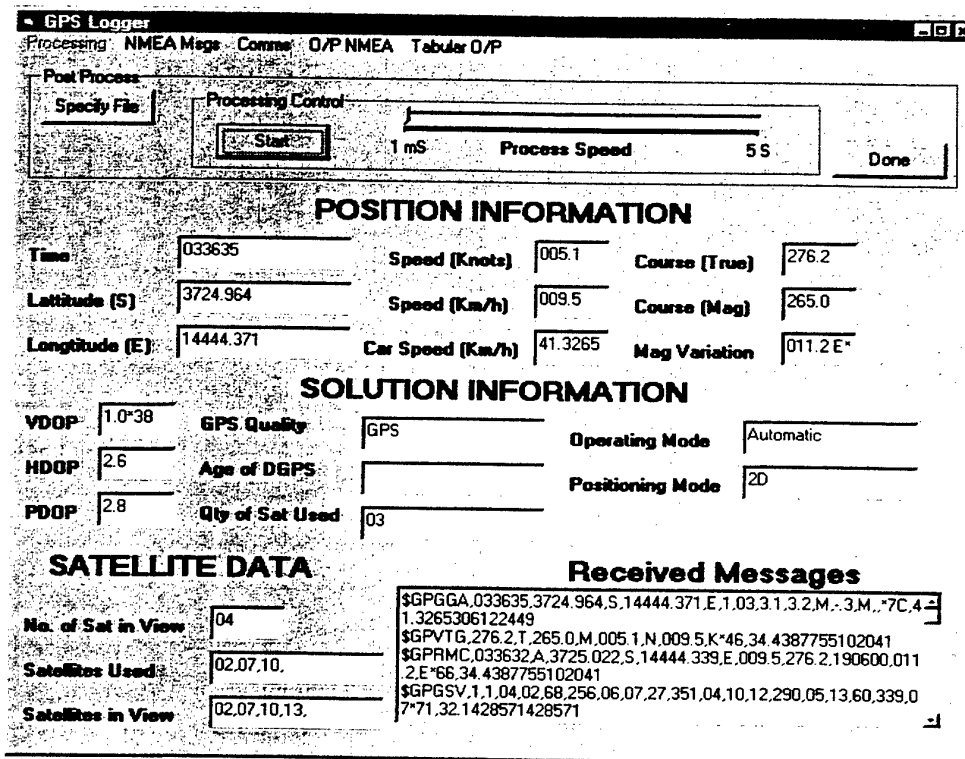
Figure 11: Screen Capture of the GPS/Velocity Logger
