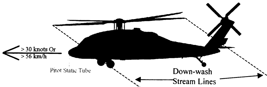
Figure 1: Speed Greater than 30 knots - Downwash has no affect on Pitot Static Tube readings
