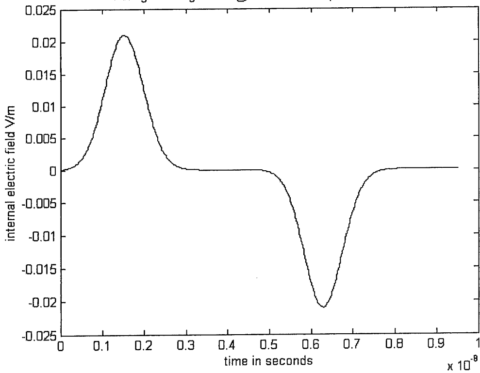
Figure 11. The response at 1.88 meter depth to the incident pulse shown in Figure 9 for Single leaf foliage.
