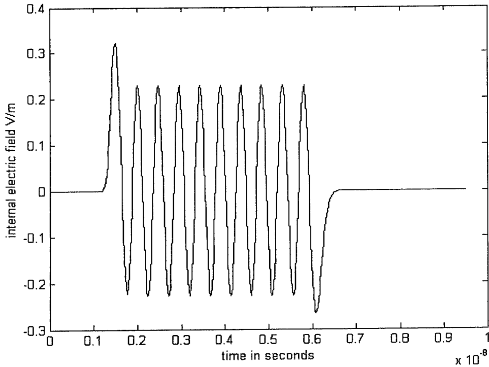
Figure 10. The response at 1.88 meter depth to the incident pulse shown in Figure 9 for Cenco Sealstix cement.
