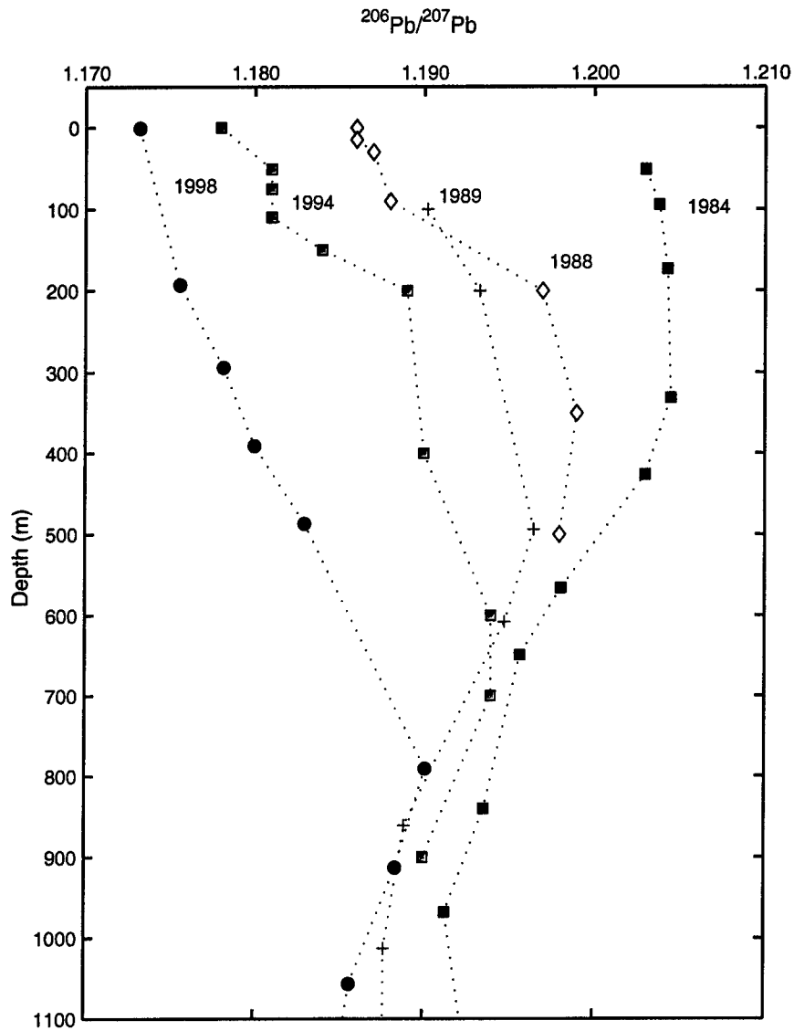
Figure 3-6: Western North Atlantic thermocline ^{206}\text{Pb}/^{207}\text{Pb} evolution, 1984 to 1998. The profile data are from Shen and Boyle (1988b, sampled in 1984 at Station S, 32^{\circ}2'\text{N} , 64^{\circ}30'\text{W} ), Sherrell et al. (1992, sampled in 1988 near Station S, 32^{\circ}0'\text{N} , 64^{\circ}10'\text{W} ), Véron et al. (1993, sampled in 1989 at BATS, 31^{\circ}5'\text{N} , 64^{\circ}1'\text{W} ), Véron et al. (1998, sampled in 1994 at BATS), and this study (sampled in 1998 at 33^{\circ}42'\text{N} , 57^{\circ}40'\text{W} ). Differences among site locations should be considered when interpreting these profiles. Note the consistent ^{206}\text{Pb}/^{207}\text{Pb} thermocline reduction and the isotopic maximum (800 meters) in the 1998 profile.
