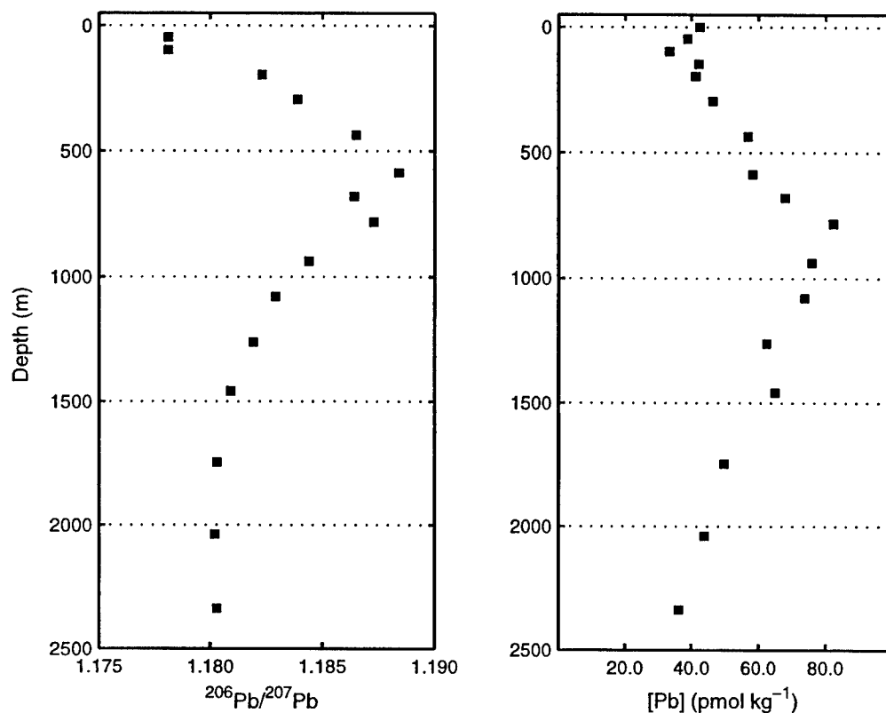
Figure 3-7: Eastern North Atlantic stable lead isotope and lead concentration profiles: Endeavor-328 , Station 7 (31°0'N, 31°0'W). The left panel reflects the ^{206}\text{Pb}/^{207}\text{Pb} ratio, and the right panel denotes total lead concentrations. Note the offset between the elemental and isotopic maxima, resulting from an 11-year phase lag between the elemental (1947-1989) and isotopic (1968-1990) North Atlantic transients.
