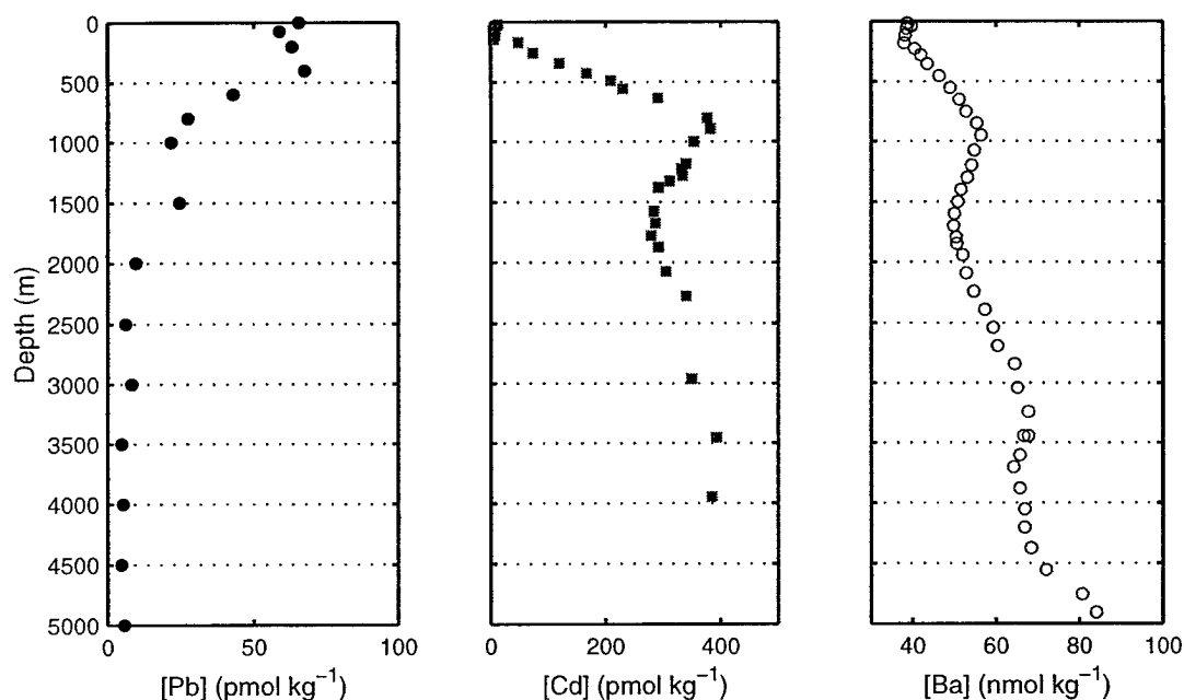
Figure 1-1: Water column profiles for cadmium, barium, and lead. The lead seawater profile, from Schaule and Patterson (1983, central northeast Pacific, 32°41'N, 145°00'W), exhibits clear particle-scavenging effects, with reduced concentrations from mixed layer to intermediate depths. The cadmium profile, from Wu and Boyle (1997b, eastern North Atlantic, 26°25'N, 33°40'W), shows a nutrient-like profile from biological uptake and remineralization. The barium profile demonstrates deeper barium regeneration from biogenic barite dissolution (Chan et al. , 1977). The secondary [Ba] maximum at 900 meters also reflects Antarctic Intermediate Water in the western North Atlantic.
