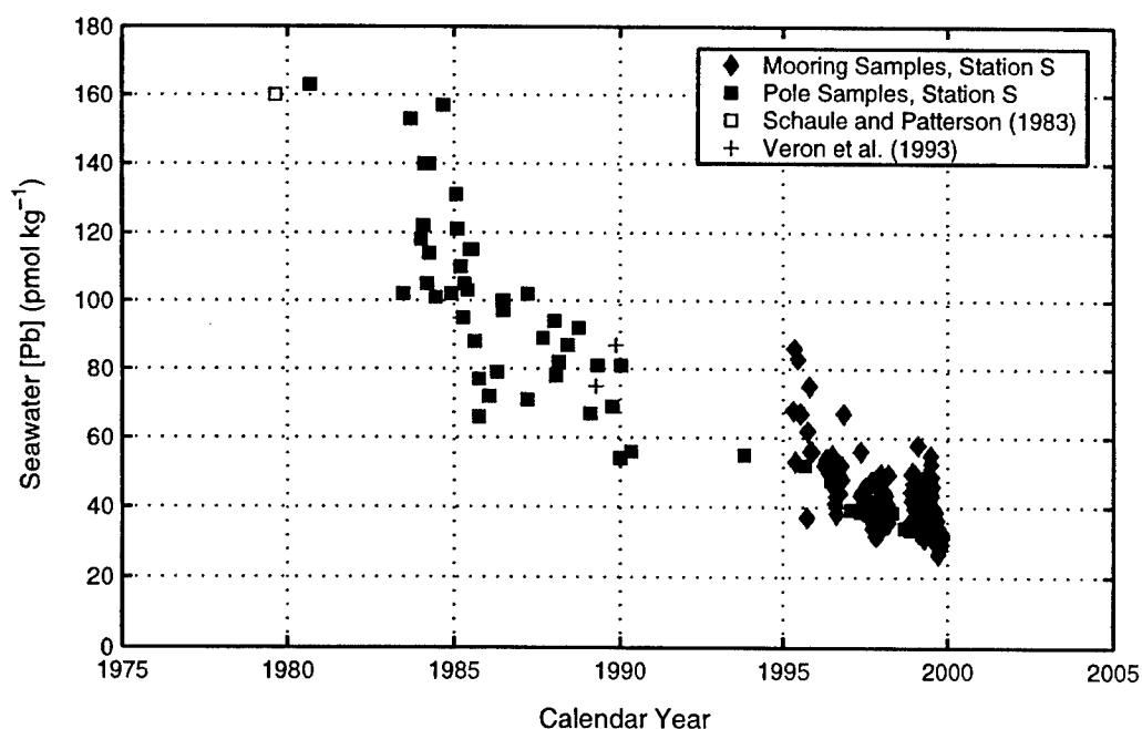
Figure 1-5: Bermuda seawater lead time series analysis, 1979-2000, adapted from Wu and Boyle (1997a). Surface mixed layer lead concentrations (in pmol kg -1 ) from Station S are shown, including results from Schaule and Patterson (1983, □) and Véron et al. (1993, +). The closed squares were collected by the pole sampling method at Station S, and closed diamonds reflect MITESS mooring samples. See Wu and Boyle (1997a) for additional details.
