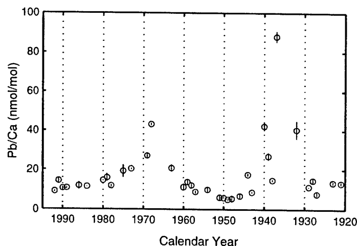
Figure 5-8: Cariaco Basin Pb/Ca record: Isla Tortuga. Note the Pb/Ca maxima at 1968 and 1937 and the good agreement among sample replicates. No systematic Pb/Ca reduction is observed at 1950. Error bars are \pm 2\sigma .
