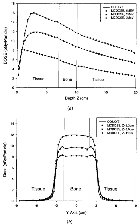
Figure 7. Dose distributions in a tissue–bone–tissue phantom calculated by DOSXYZ and MCDOSE for 6 MeV, 15 MV and 2 MeV photon beams with field size of 6 cm × 6 cm defined at 100 cm SSD. The material in the volume of –5.0 cm to 5.0 cm along the X direction, –2.0 cm to 2.0 cm along the Y direction and 7.0 cm to 10.0 cm along the Z direction is bone. (a) The depth dose curve along the central axis for the beams. (b) The lateral dose profiles along the Y axis at depths of 3.3 cm, 8.0 cm and 11.0 cm for the 15 MV photon beam.
