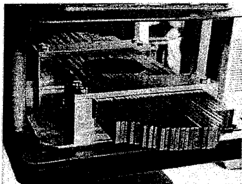
Figure 1. A prototype of an electron MLC mounted on the bottom scraper of a 25 cm \times 25 cm applicator on a Varian Clinac 2100C accelerator. The MLC has 30 pairs of steel leaves and the leaf positions are fixed by the tightening screws.
