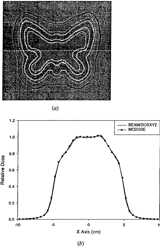
Figure 5. (a) is the isodose distributions in XY view at a depth of 2.25 cm in a water phantom for a modified 10 cm × 10 cm 12 MeV electron beam using an electron cutout with a butterfly-shaped opening. The thick curve is the simulation result of BEAM/DOSXYZ. The thin curve is the result of MCDOSE. (b) The lateral dose profile along the dashed line in (a). The curve with symbols in (b) is the result of MCDOSE.
