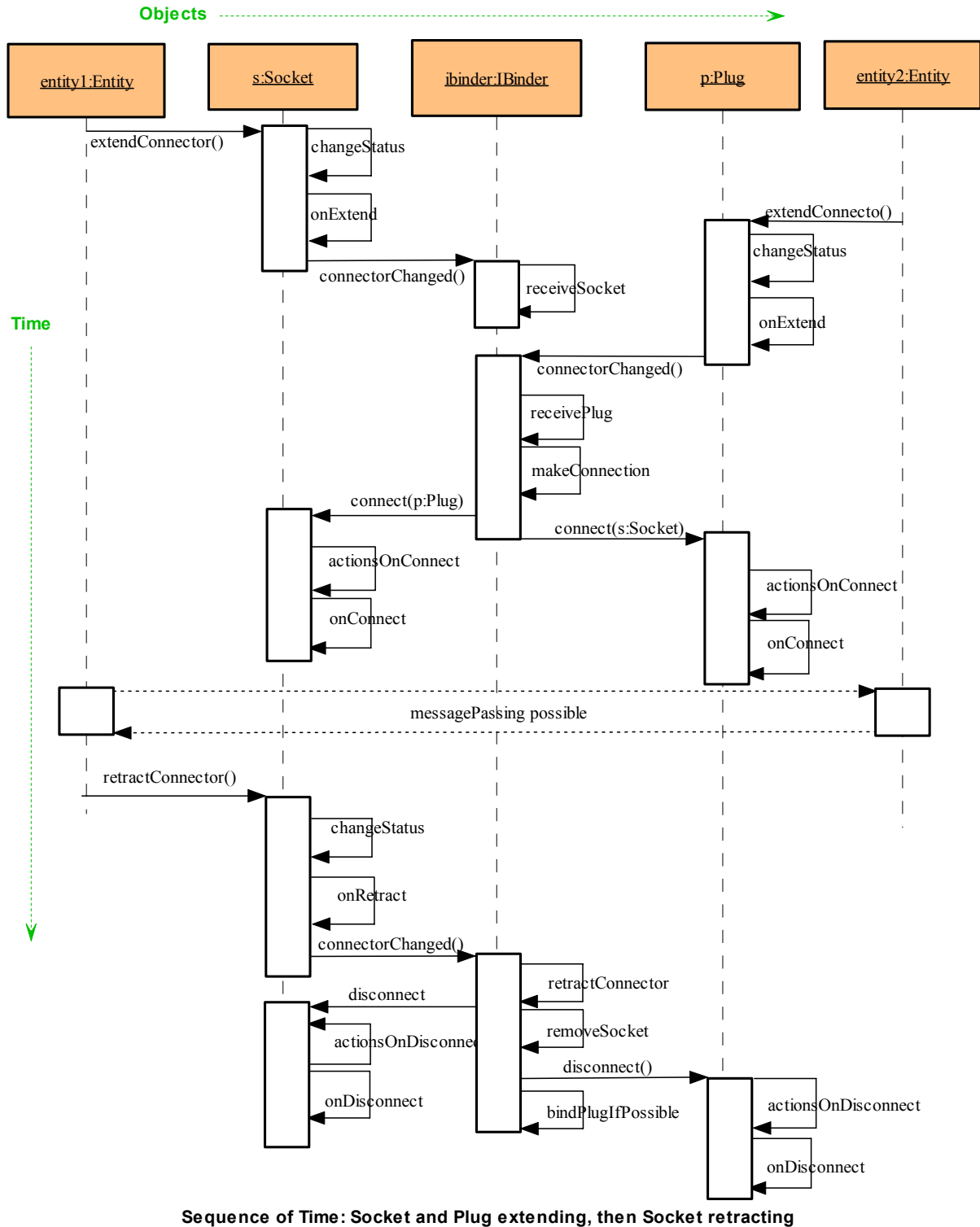
Figure 22. A sequence diagram of Socket and Plug connecting and disconnecting over time.
