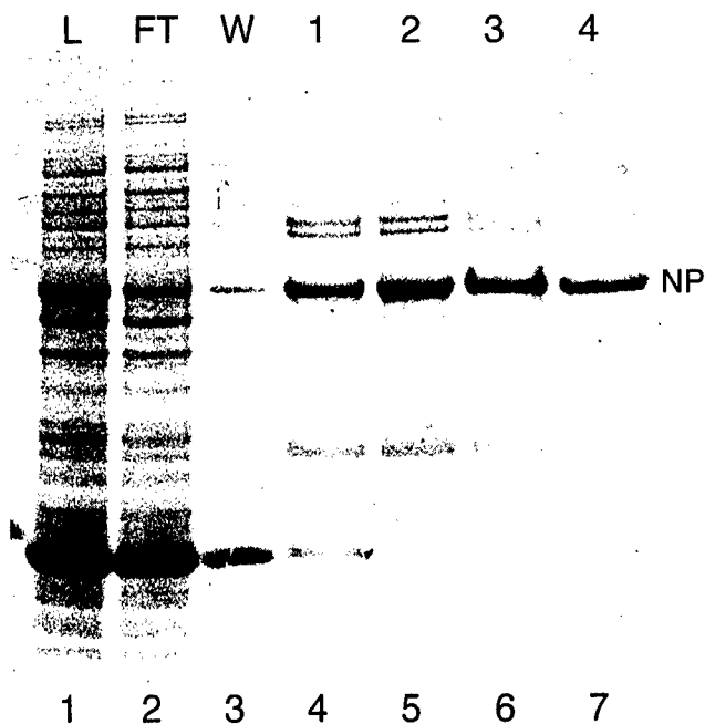
FIG. 2. Native purification of the SNV N protein by Ni-NTA chromatography without Chaps. A representative purification from cellular material extracted without Chaps is shown. L, column load; F, column flowthrough; W, column wash; 1–4, fractions eluted from column. These samples were subjected to separation by 4–12% NuPAGE Novex Bis-Tris gels.
