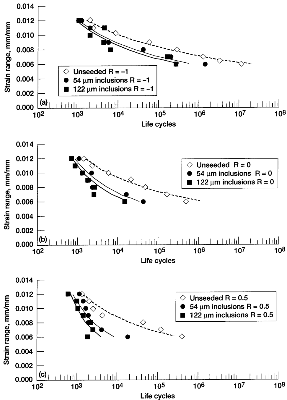
Figure 3.—LCF lives of unseeded versus seeded disk specimens. Estimates of the regression model are also shown. (a) R_e = -1 . (b) R_e = 0 . (c) R_e = 0.5 .
