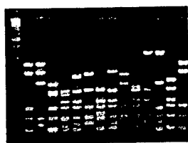
Fig. 3. DNA fingerprint analysis of the scFv genes of individual antibodies from the second round of selection. scFv DNA was amplified by PCR directly from colonies and digested with the frequently cutting restriction enzyme Bst NI. A diverse banding pattern was observed, with each unique pattern representing a unique antibody sequence. First lane is a 100-bp DNA marker.
