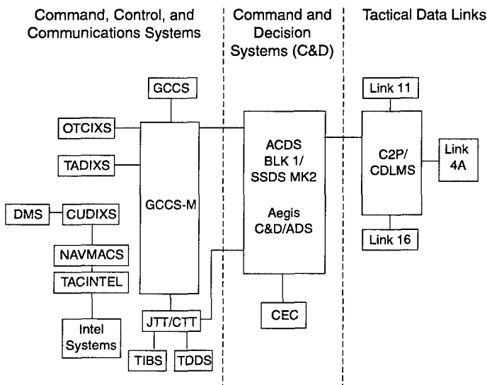
FIGURE 3.9 BMC3 system architecture. DMS, defense message system; OTCIXS, officer in tactical command information exchange subsystem; TADIXS, tactical data information exchange system; CUDIIXS, common user data information exchange system; NAVMACS, naval modular automated communications system; TACINTEL, tactical intelligence information exchange system; JTT, joint tactical terminal; CTT, commander's tactical terminal; TIBS, tactical information broadcast service; TDDS, tactical receive applications (TRAP) data dissemination system; ADS, advanced display system; CDLMS, common data link management system.
