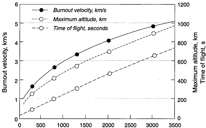
FIGURE 2.2 Minimum burnout velocity, maximum altitude, and time of flight as functions of range between burnout and reentry. Burnout altitude = reentry altitude = 10 km with Earth's rotation and atmospheric effects neglected. NOTE: This figure is approximate and actual values will vary according to more detailed scenarios. SOURCE: Calculations based on (1) Bate, Roger R., Donald D. Mueller, and Jerry E. White, 1971, Fundamentals of Astrodynamics , Dover Publications, Mineola, N.Y.; Thomson, W.T., 1961, Introduction to Space Dynamics , Dover Publications, Inc., Mineola, N.Y., December; (2) Thomson, William T., 1961, Introduction to Space Dynamics , Dover Publications, Mineola, N.Y., paperback edition, May 1986; (3) Sellers, Jerry J., and Wiley J. Larson, 1961, Understanding Space: An Introduction to Astronautics , Space Technology Series, McGraw-Hill, New York, N.Y.; and (4) Sellers, Jerry J., William J. Store, Robert B. Giffen, and Wiley J. Larson, 2000, Understanding Space: An Introduction to Astronautics , 2nd edition, McGraw-Hill College Division, McGraw-Hill, New York, N.Y., June.
