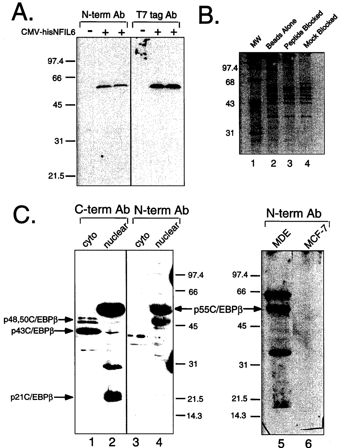
Fig. 3. Characterization of the N-terminal human C/EBP \beta -1 antibody. A: NIH 3T3 cells were transfected with 8 \mu g of a CMV-driven histagged NFIL6 expression vector modified so that only protein initiating at the first ATG would be produced (+) or control CMV-4 vector (-). Cells were harvested 40 h post-transfection and whole cell extracts prepared and analyzed as in Figure 2. Immunoblotting was performed with the N-terminal C/EBP \beta or an antibody to the T7 histidine tag (Novagen). B: ^{35} S methionine-labeled whole cell extracts from HMEC cells were incubated with agarose beads alone (lane 2), beads plus N-terminal antibody (lane 3), or beads plus N-terminal antibody pre-blocked with 700 ng of N-terminal peptide (lane 4).
