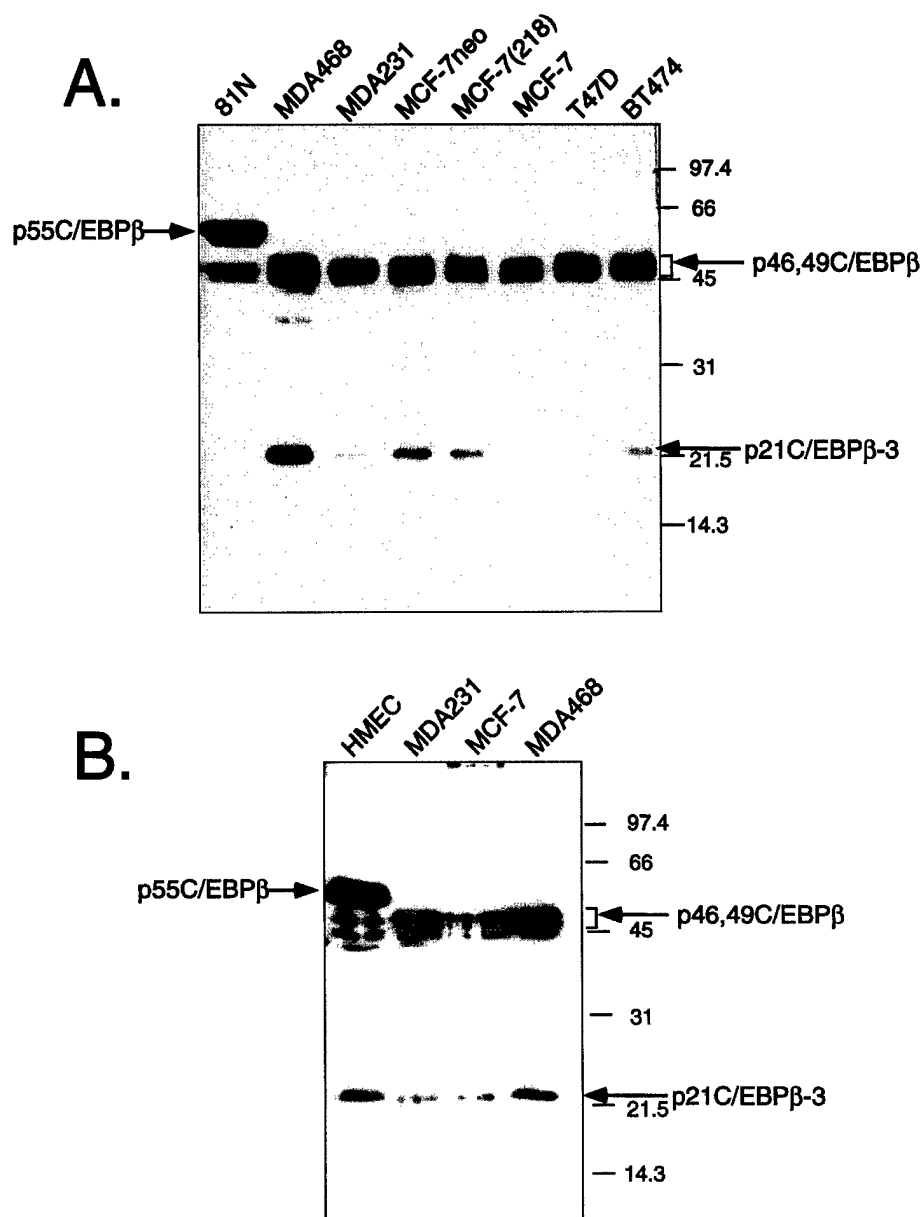
Fig. 2. Breast cancer cell lines display a different pattern of C/EBP \beta expression than normal cells. A: Whole cell extracts were made from a battery of breast cancer cell lines as well as from a population of normal cells, 81N. Equal amounts of total cell protein were analyzed by SDS-12% polyacrylamide gel electrophoresis. Immunoblotting was
