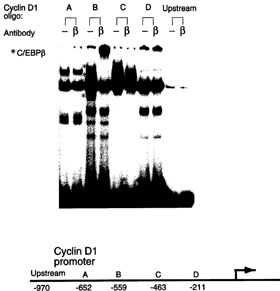
Fig. 7. C/EBP \beta will bind the -559 site in the cyclin D1 promoter. Radiolabeled oligonucleotides representing potential C/EBP \beta binding sites in the cyclin D1 promoter as depicted in the diagram were incubated with either nuclear extracts from MDA 231 cells or extracts pre-mixed with C-terminal C/EBP \beta antibody. Reactions were
