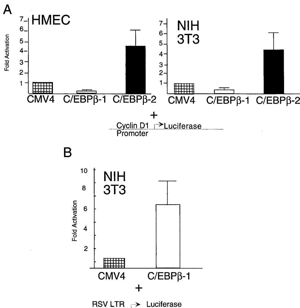
Fig. 8. C/EBP \beta -2, but not C/EBP \beta -1, will activate the cyclin D1 promoter. A: HMECs were transfected for 5 h with 2 \mu g of the cyclin D1/luciferase construct (pGL3cycD) and 2 \mu g of empty vector (CMV4) or 2 \mu g of expression vector for either C/EBP \beta -1 or C/EBP \beta -2 using Geneporter liposomes. NIH 3T3 cells were transfected for 8 h with
