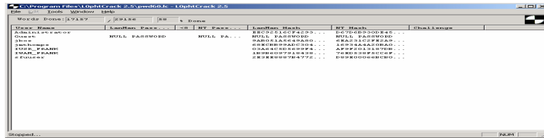
Figure 4.2 L0phtCrack 2.5
