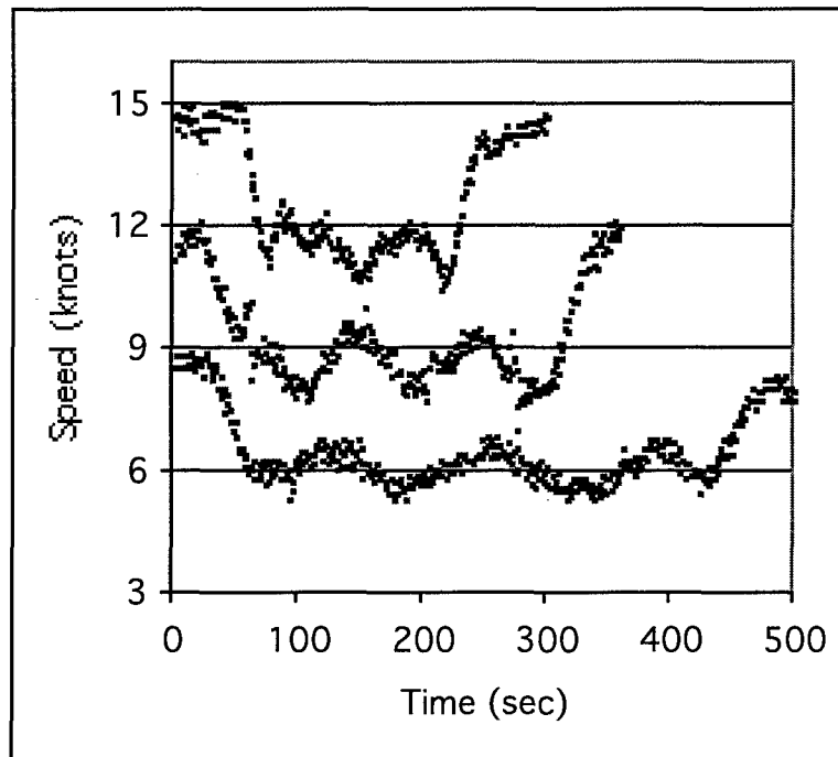
Figure G.11 Sea Trial Port 30 (0.72)
