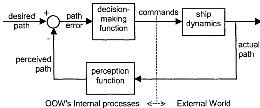
Figure 1 PCT Model of Ship Manoeuvres under the Control of the OOW
