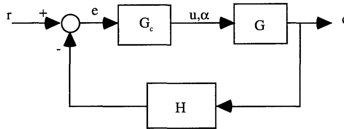
Figure 2 Standard Feedback Control System
