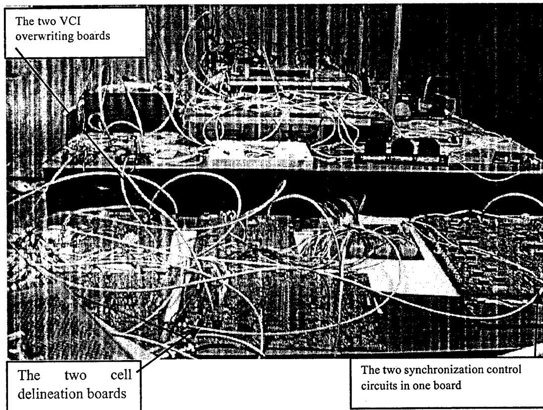
Fig. 39 Experimental setup
