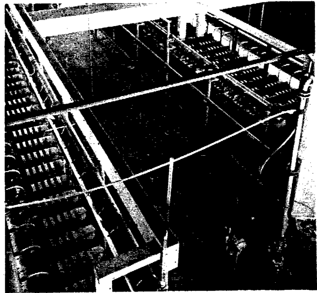
Figure 9. Los Angeles \text{KClO}_4 Plant Sodium Perchlorate Cells 2500 Amps
