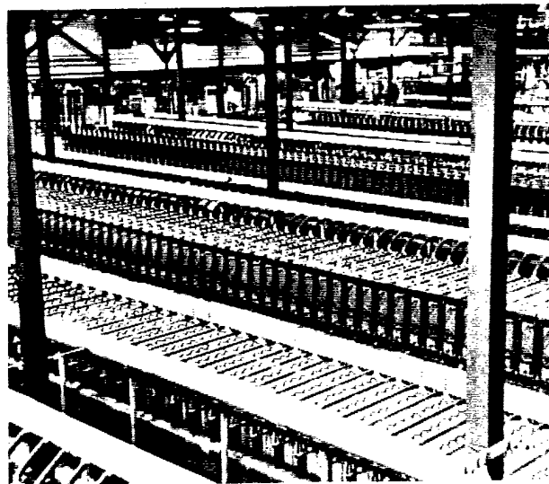
Figure 12. WECCO Henderson, Nevada \text{KClO}_4 Plant 5000 Amp Electrolytic Chlorate and Perchlorate Cell Room
