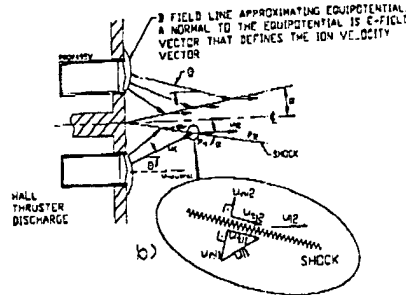
Fig. 11 Similarities between oblique shock in supersonic flow and jet mode shock cone at the exit of a Hall thruster
