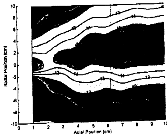
Fig. 13 Typical plasma potential color contour map
