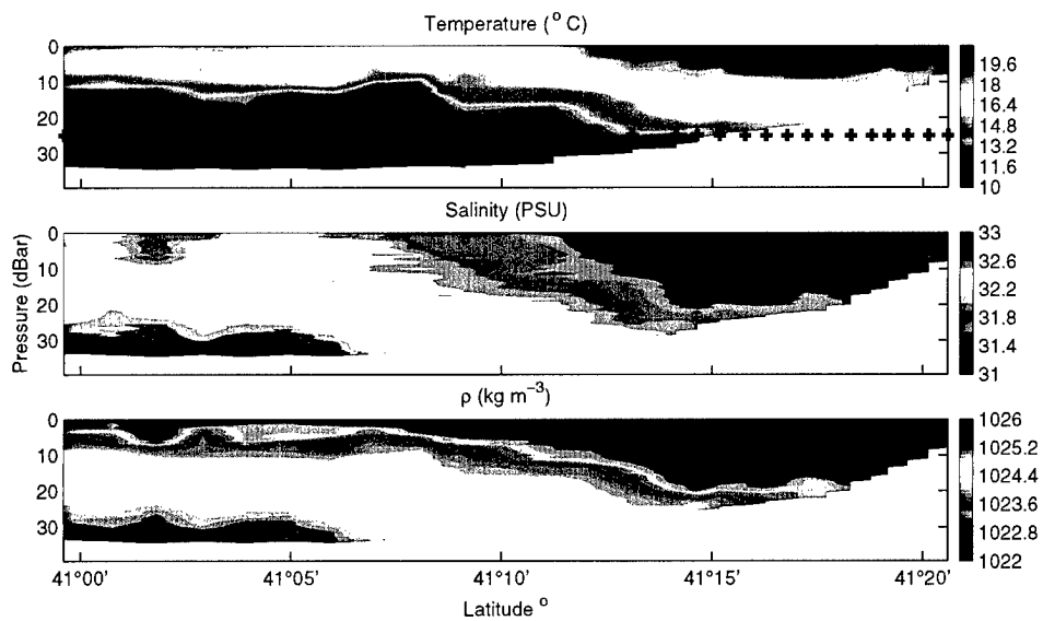
Figure 28: An example of a CTD survey recorded on an across shelf transect during the CBLAST-Low 2001 IOP.
