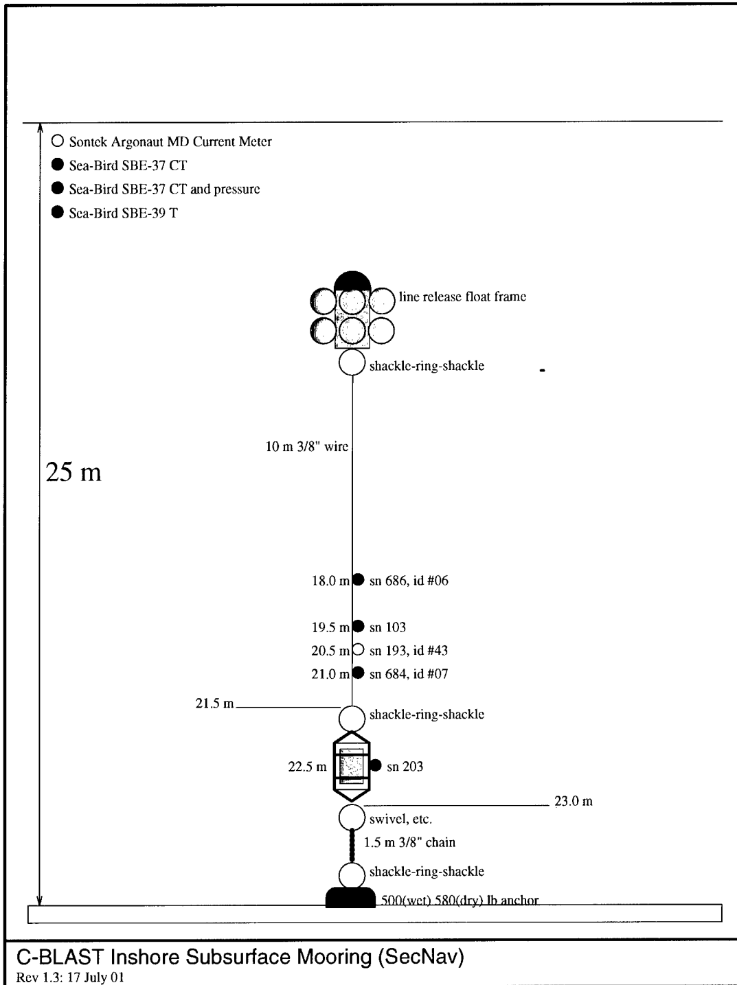
Figure 5b: Schematic diagram of SecNav subsurface mooring.
