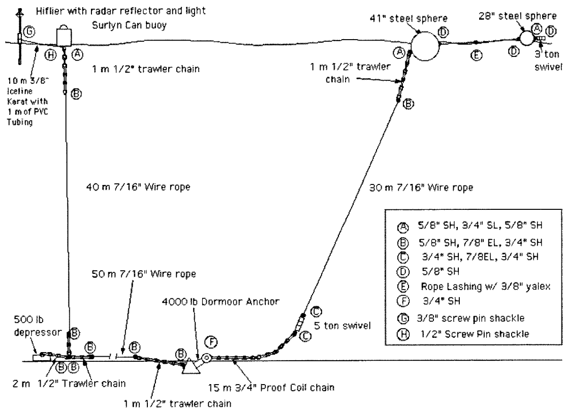
Figure 11a: CBLAST-Low three-dimensional net corner mooring and tensioning hardware.
