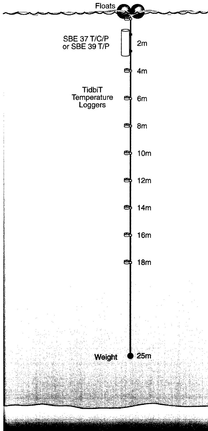
Figure 6: Artists impression of a three-dimensional net vertical string array with attached instrumentation for the CBLAST-Low 2001 pilot experiment.
