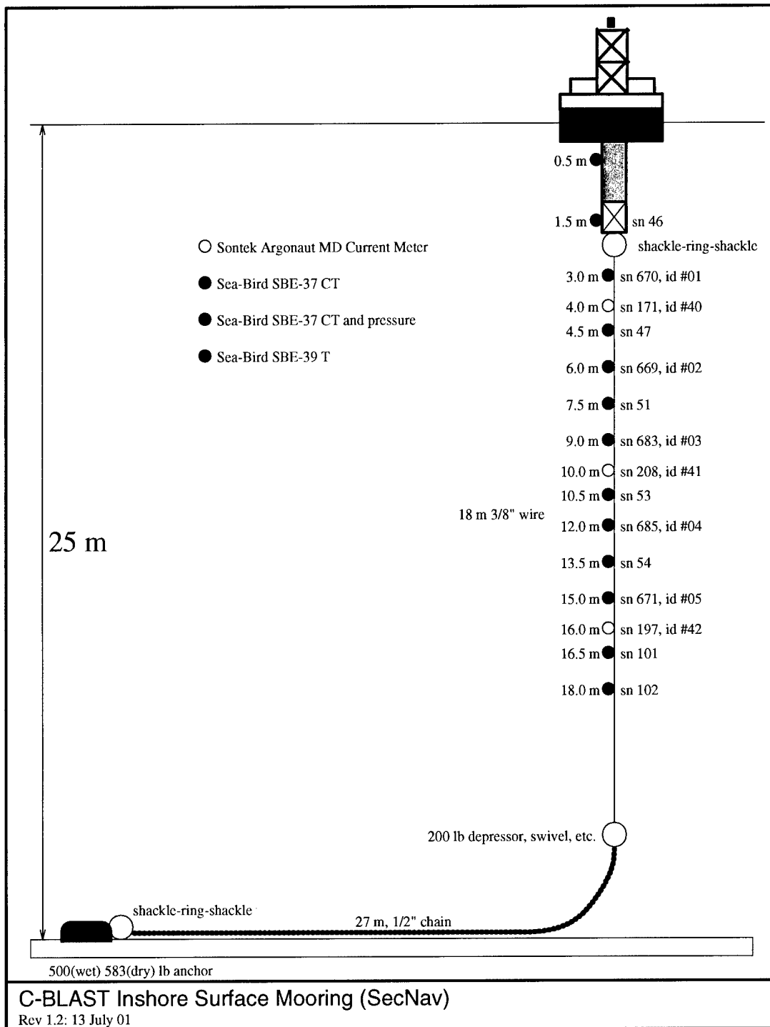
Figure 5a: Schematic diagram of SecNav surface mooring
