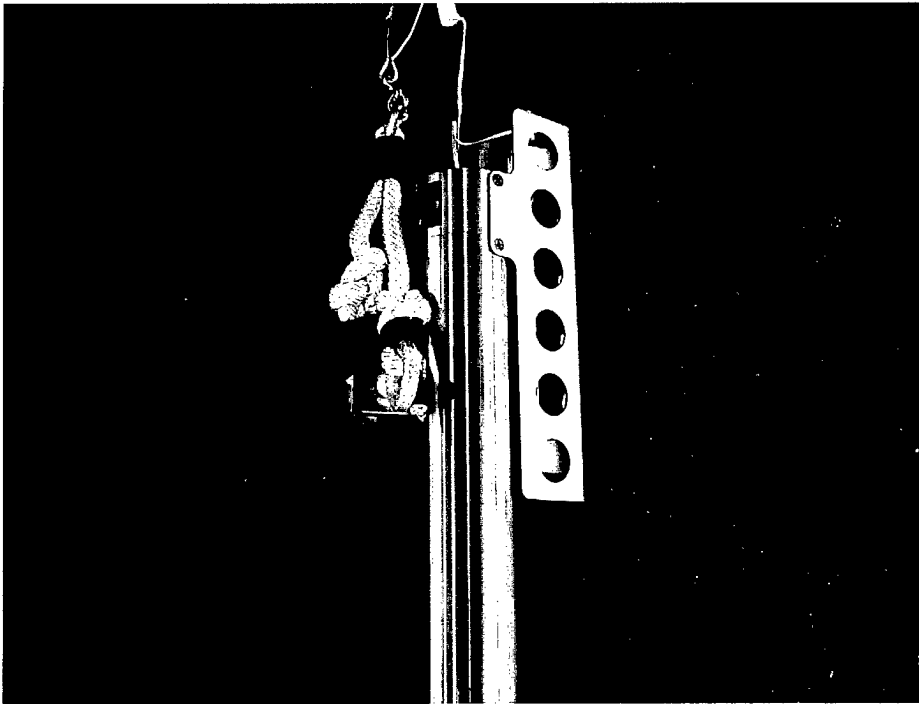
Figure 9: Photograph of the rigging method for SBE 37 temperature/conductivity recorders used on the three-dimensional array.
