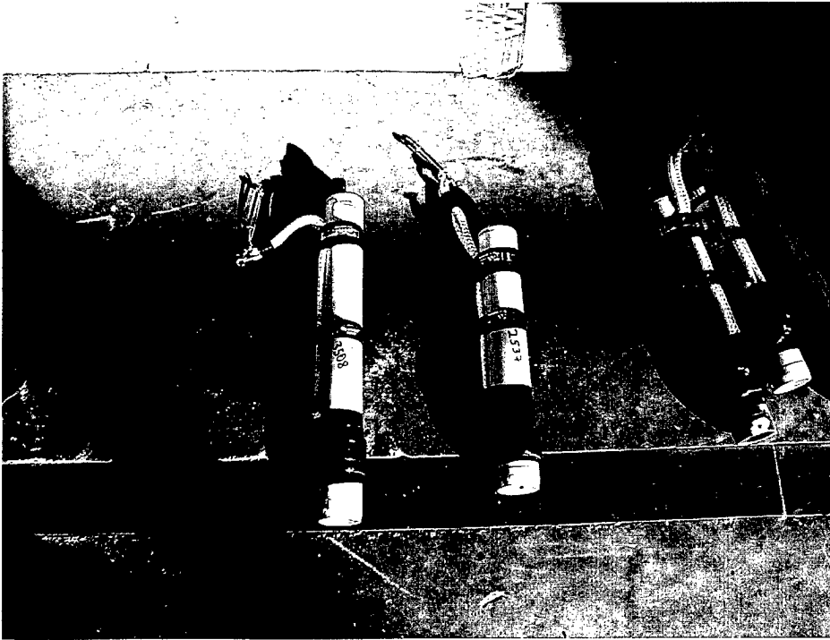
Figure 8: Photograph of the rigging method for Brancker temperature loggers used on the three-dimensional array.
