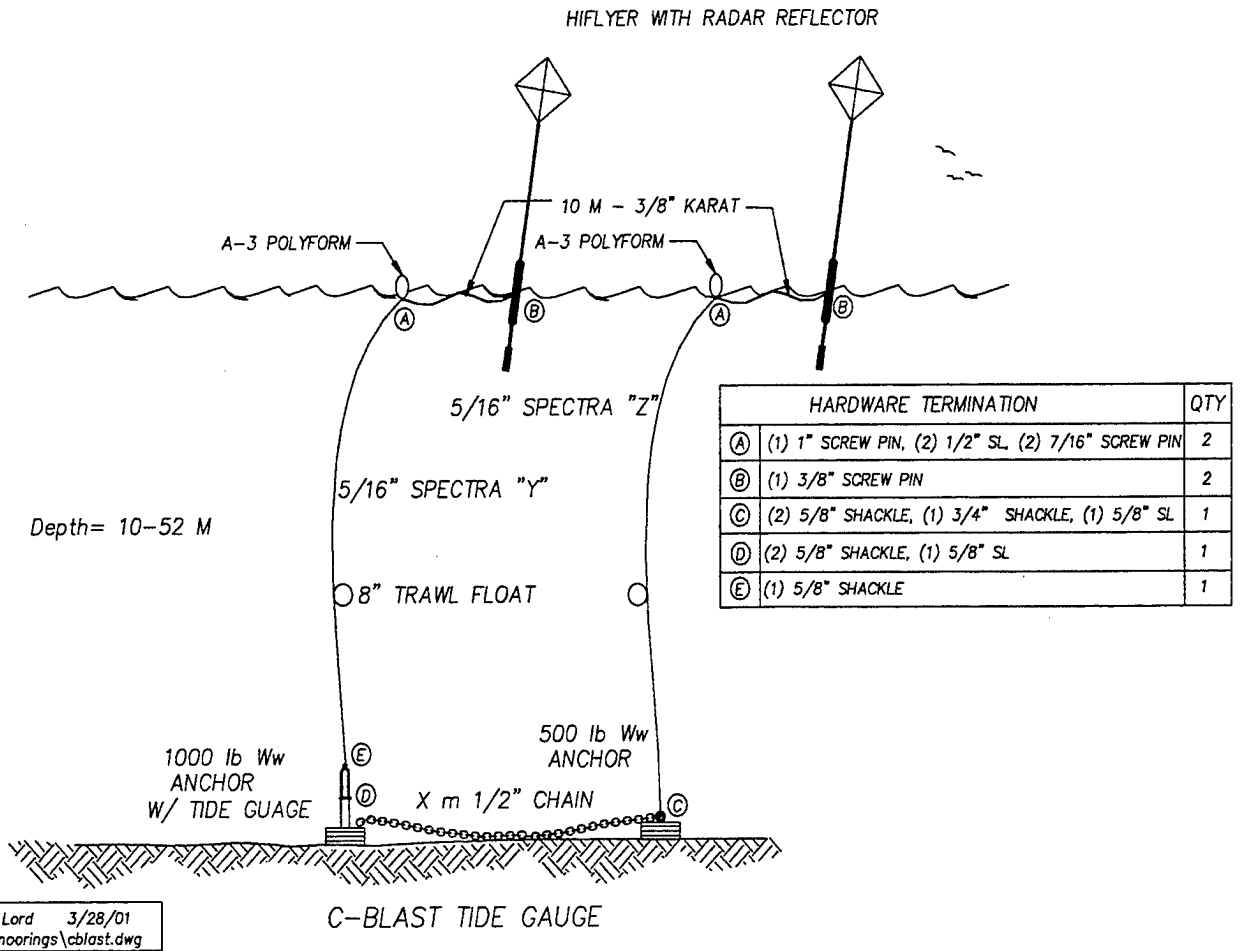
Figure 2: Schematic diagram of the tide gauge mooring hardware used during the CBLAST-Low 2001 pilot study.
