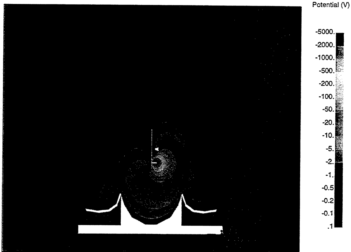
Figure 16. Potentials and sample trajectories for the WSF in the shuttle wake with the wake side probe at -5000\text{ V} in a 10^{11} , 0.1\text{ eV} plasma, moving at 7800\text{ m s}^{-1} as computed by DynaPAC.
