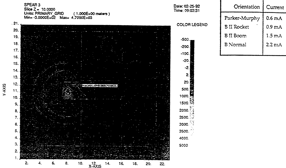
Figure 2. DynaPAC calculated electrostatic potentials about SPEAR-3, illustrating a case of weak sheath overlap.
