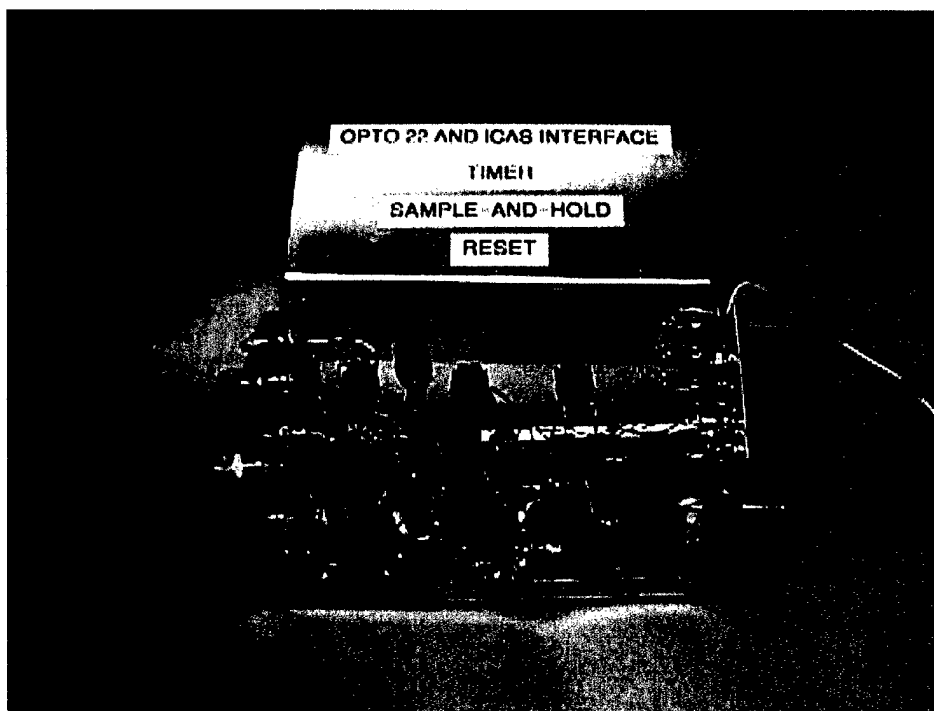
Figure 23. One-Second Data Sample and Reset circuit [9A] and photo.
