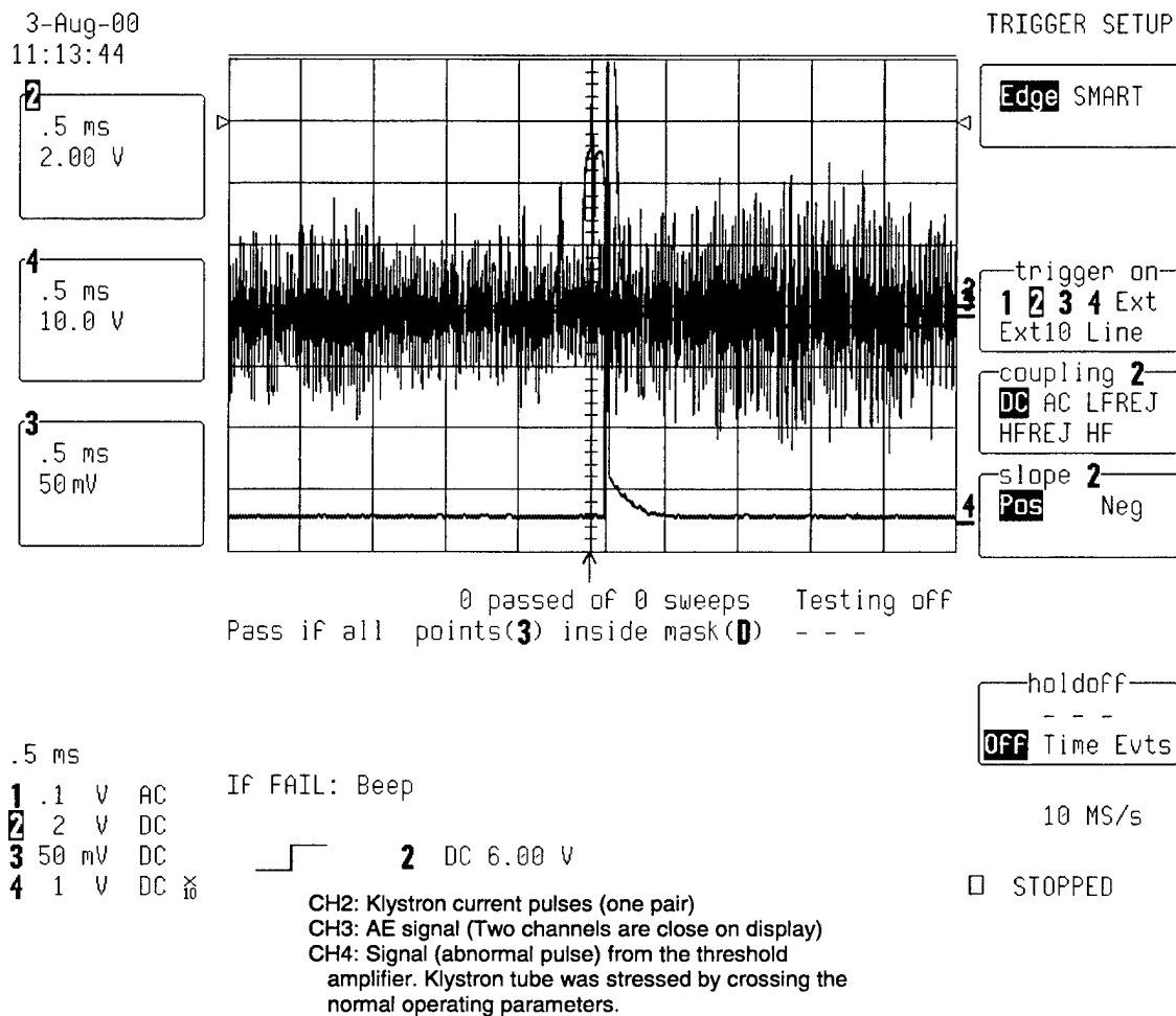
Figure 7. Abnormal current pulse is caught on Ch4 AN/SPS-49 radar klystron unit at NSW PHD Dam Neck.
